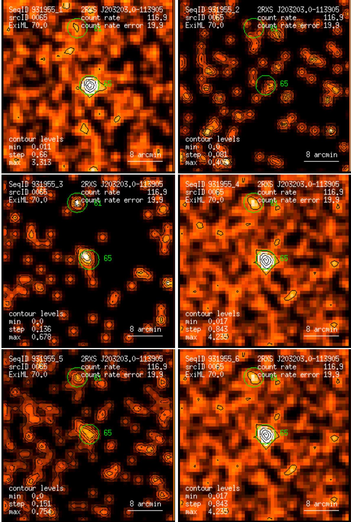
Figure 65: RASS 931955: detection 0065: band rate images, Gaussian filter: (1) PSPC channels 11 – 41, (2) 52 – 90, (3) 91 – 201, (4) 11 – 235, (5) 52 – 201, (6) 11 – 201. Broad band rates in counts/ks. Band rate contour levels in counts/ks/arcmin 2 .
