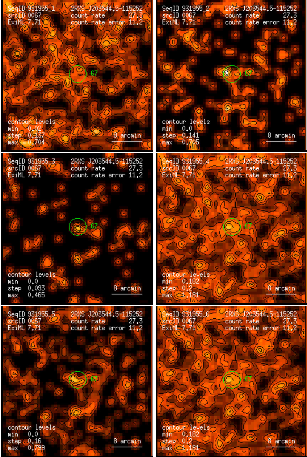
Figure 67: RASS 931955: detection 0067: band rate images, Gaussian filter: (1) PSPC channels 11 – 41, (2) 52 – 90, (3) 91 – 201, (4) 11 – 235, (5) 52 – 201, (6) 11 – 201. Broad band rates in counts/ks. Band rate contour levels in counts/ks/arcmin 2 .
