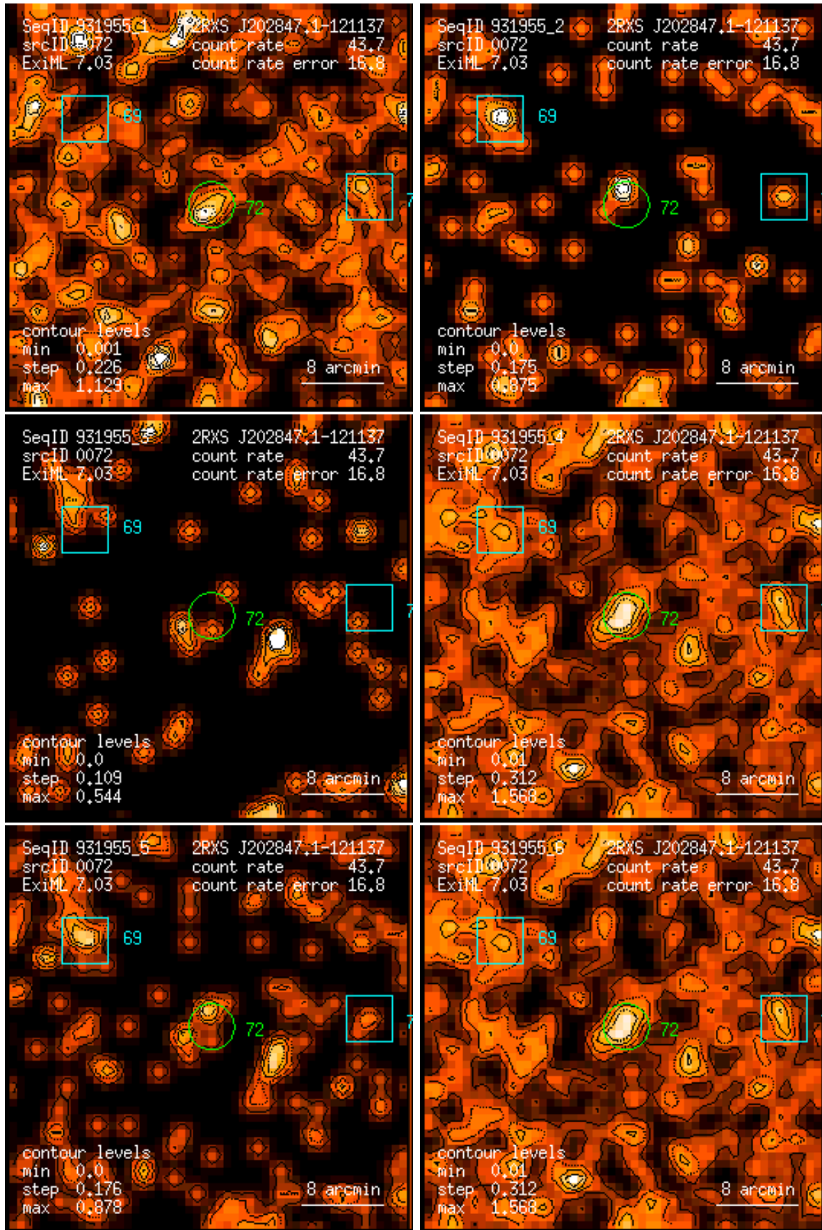
Figure 72: RASS 931955: detection 0072: band rate images, Gaussian filter: (1) PSPC channels 11 – 41, (2) 52 – 90, (3) 91 – 201, (4) 11 – 235, (5) 52 – 201, (6) 11 – 201. Broad band rates in counts/ks. Band rate contour levels in counts/ks/arcmin 2 .
