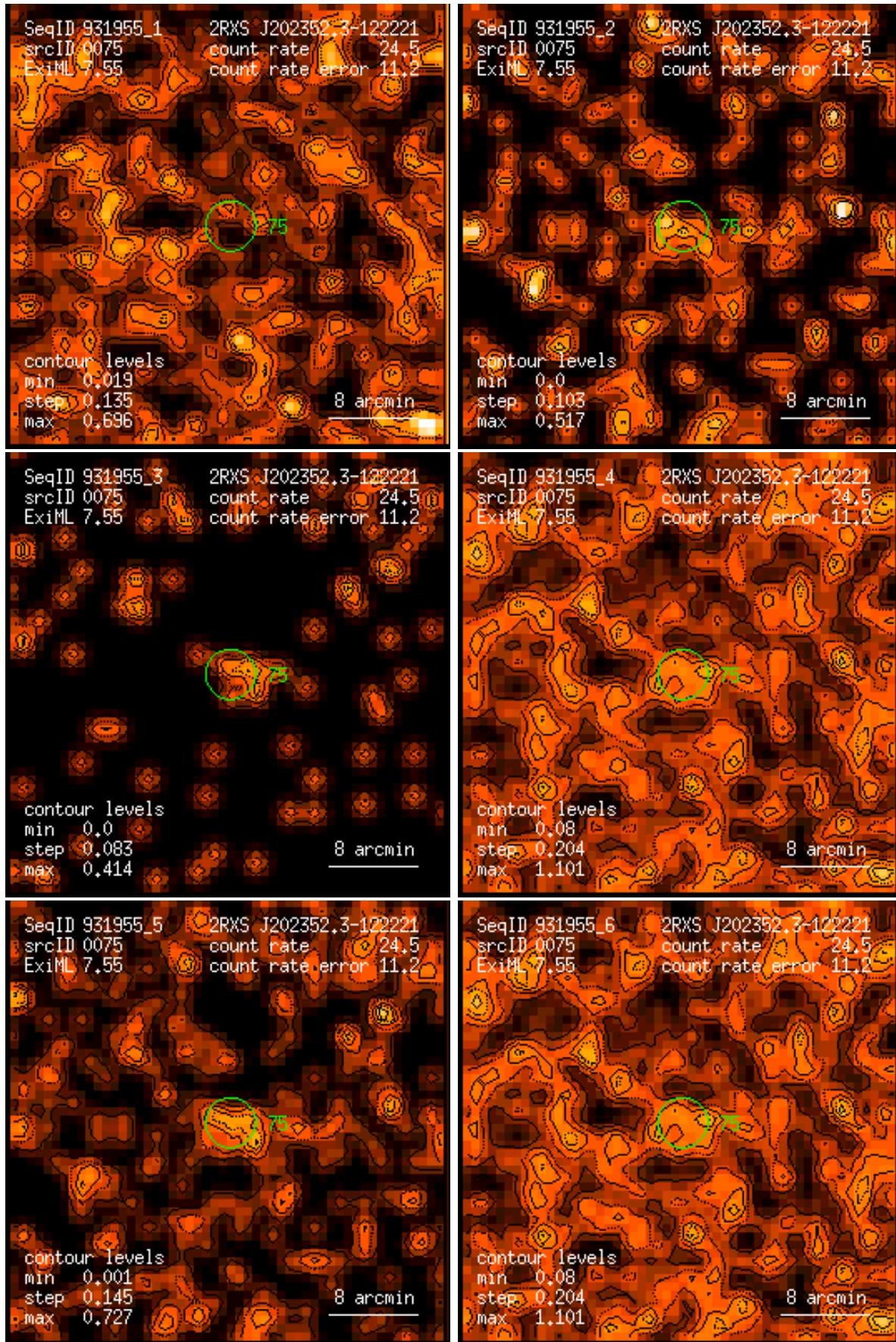
Figure 75: RASS 931955: detection 0075: band rate images, Gaussian filter: (1) PSPC channels 11 – 41, (2) 52 – 90, (3) 91 – 201, (4) 11 – 235, (5) 52 – 201, (6) 11 – 201. Broad band rates in counts/ks. Band rate contour levels in counts/ks/arcmin 2 .
