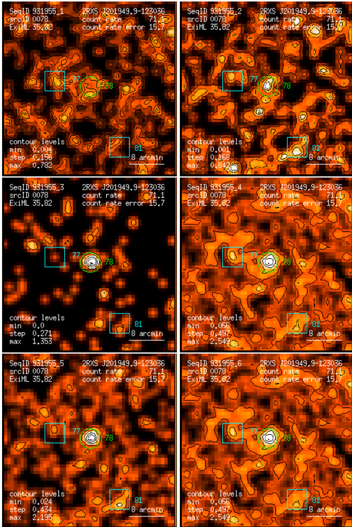
Figure 78: RASS 931955: detection 0078: band rate images, Gaussian filter: (1) PSPC channels 11 – 41, (2) 52 – 90, (3) 91 – 201, (4) 11 – 235, (5) 52 – 201, (6) 11 – 201. Broad band rates in counts/ks. Band rate contour levels in counts/ks/arcmin 2 .
