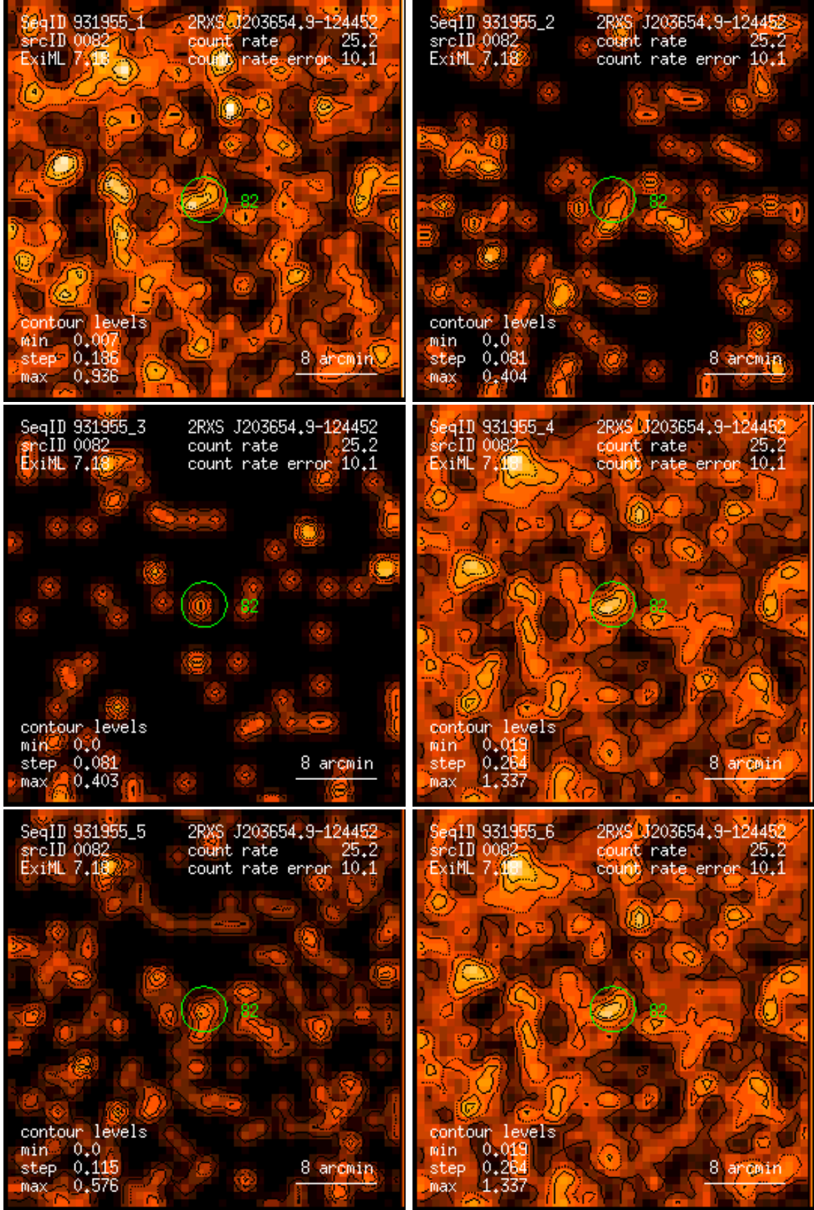
Figure 82: RASS 931955: detection 0082: band rate images, Gaussian filter: (1) PSPC channels 11 – 41, (2) 52 – 90, (3) 91 – 201, (4) 11 – 235, (5) 52 – 201, (6) 11 – 201. Broad band rates in counts/ks. Band rate contour levels in counts/ks/arcmin 2 .
