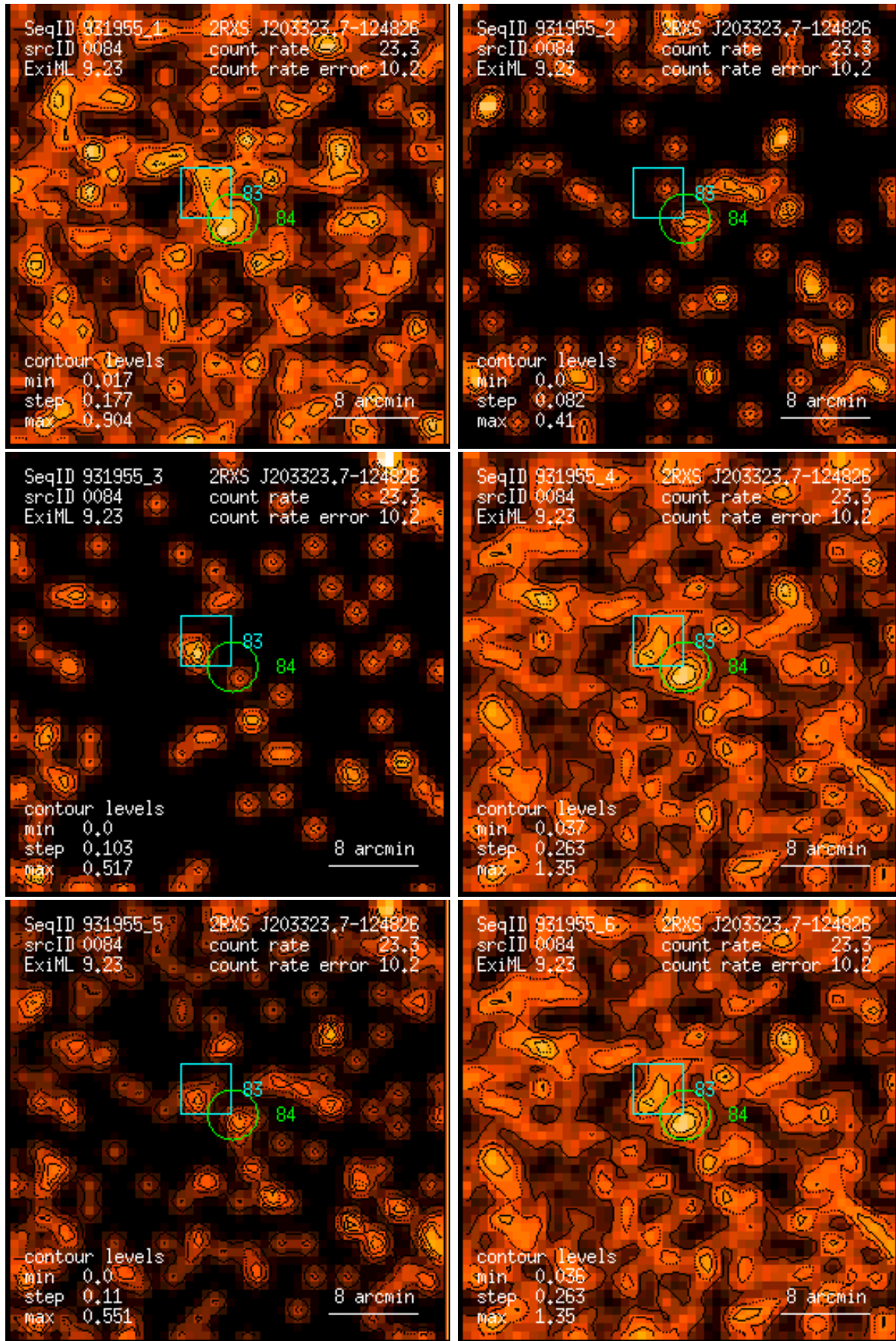
Figure 84: RASS 931955: detection 0084: band rate images, Gaussian filter: (1) PSPC channels 11 – 41, (2) 52 – 90, (3) 91 – 201, (4) 11 – 235, (5) 52 – 201, (6) 11 – 201. Broad band rates in counts/ks. Band rate contour levels in counts/ks/arcmin 2 .
