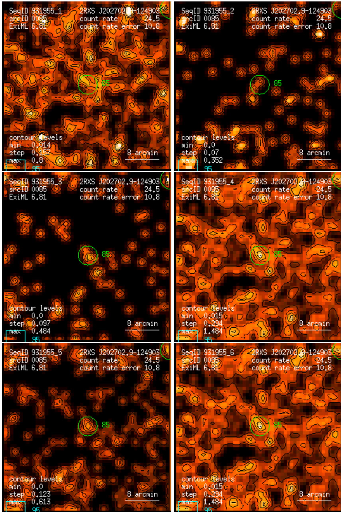
Figure 85: RASS 931955: detection 0085: band rate images, Gaussian filter: (1) PSPC channels 11 – 41, (2) 52 – 90, (3) 91 – 201, (4) 11 – 235, (5) 52 – 201, (6) 11 – 201. Broad band rates in counts/ks. Band rate contour levels in counts/ks/arcmin 2 .
