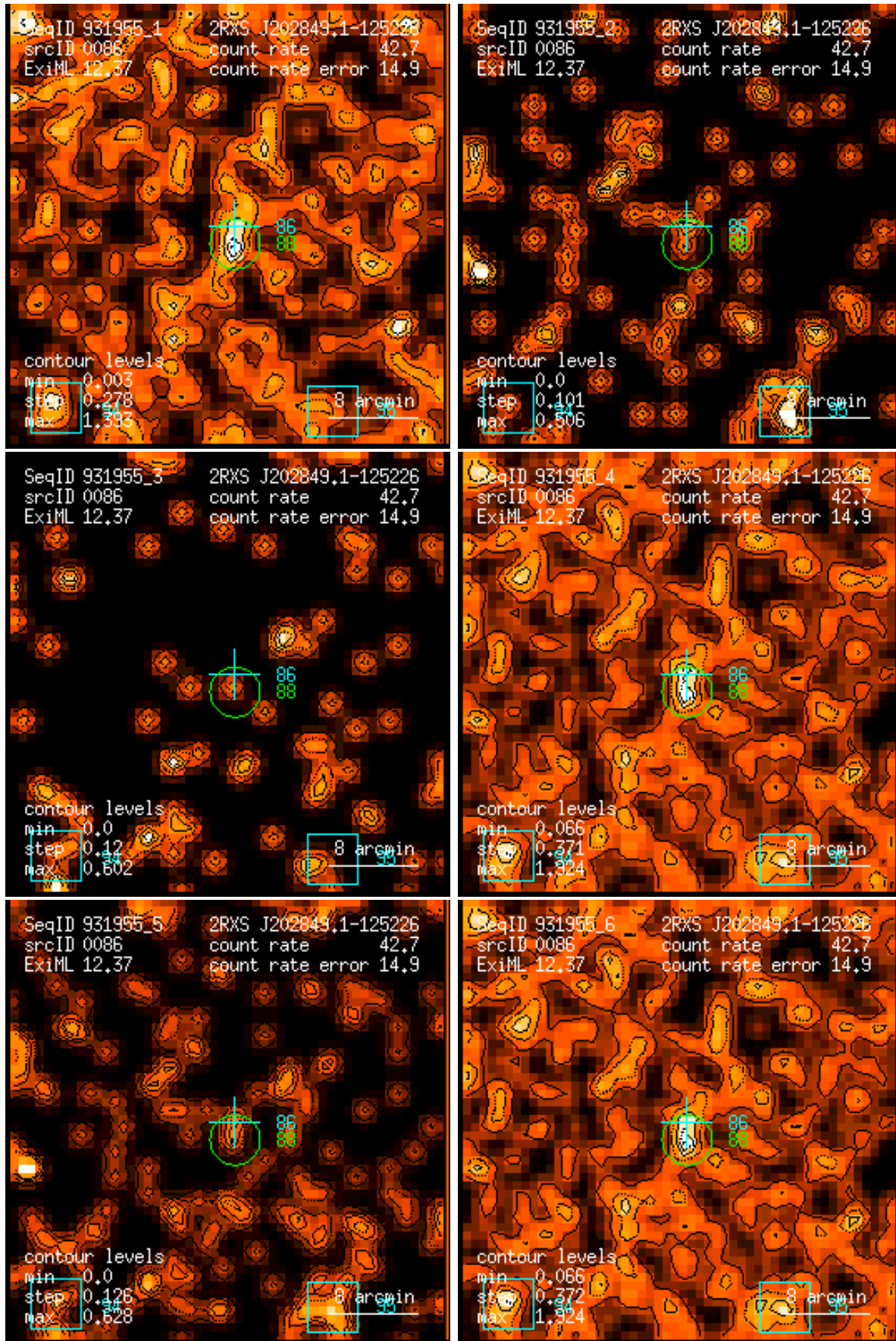
Figure 86: RASS 931955: detection 0086: band rate images, Gaussian filter: (1) PSPC channels 11 – 41, (2) 52 – 90, (3) 91 – 201, (4) 11 – 235, (5) 52 – 201, (6) 11 – 201. Broad band rates in counts/ks. Band rate contour levels in counts/ks/arcmin 2 .
