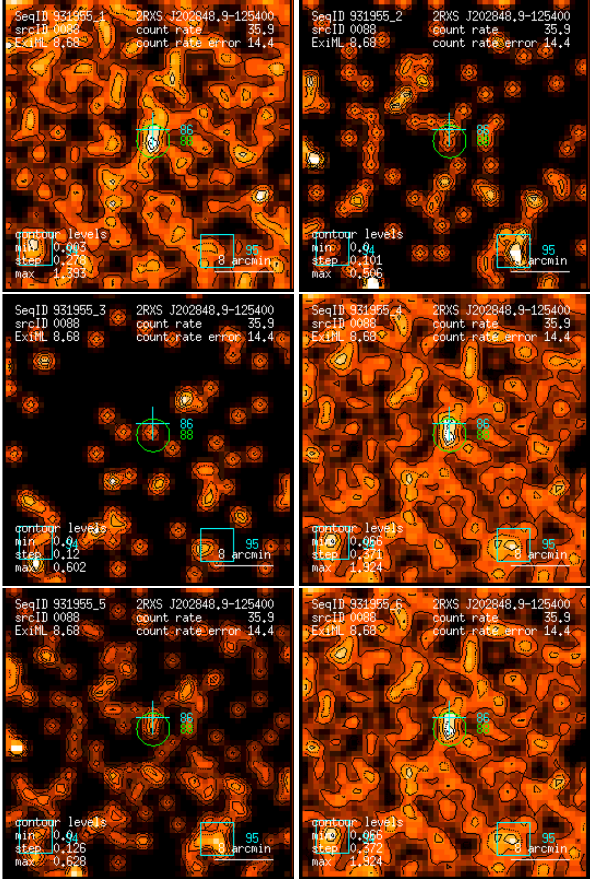
Figure 88: RASS 931955: detection 0088: band rate images, Gaussian filter: (1) PSPC channels 11 – 41, (2) 52 – 90, (3) 91 – 201, (4) 11 – 235, (5) 52 – 201, (6) 11 – 201. Broad band rates in counts/ks. Band rate contour levels in counts/ks/arcmin 2 .
