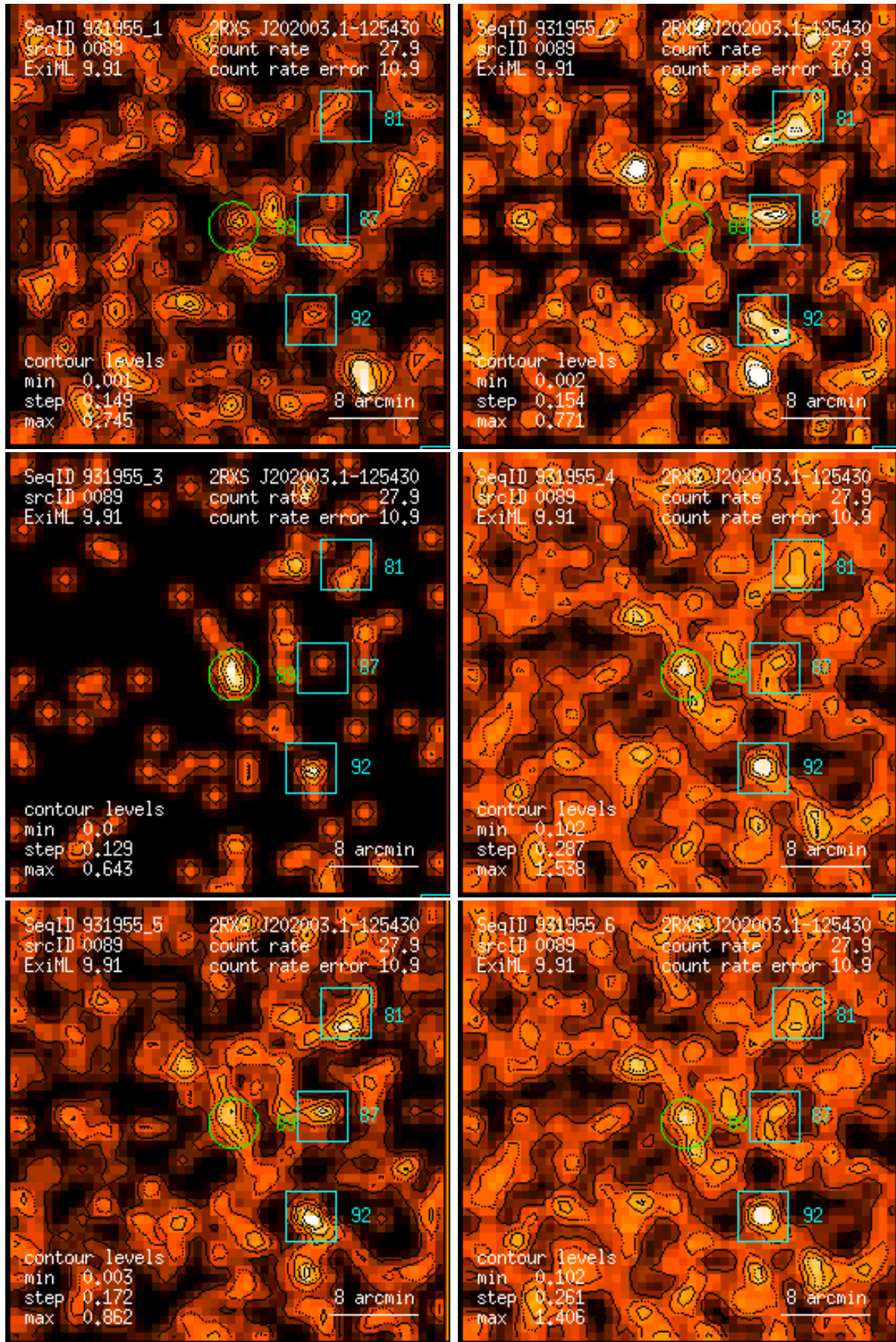
Figure 89: RASS 931955: detection 0089: band rate images, Gaussian filter: (1) PSPC channels 11 – 41, (2) 52 – 90, (3) 91 – 201, (4) 11 – 235, (5) 52 – 201, (6) 11 – 201. Broad band rates in counts/ks. Band rate contour levels in counts/ks/arcmin 2 .
