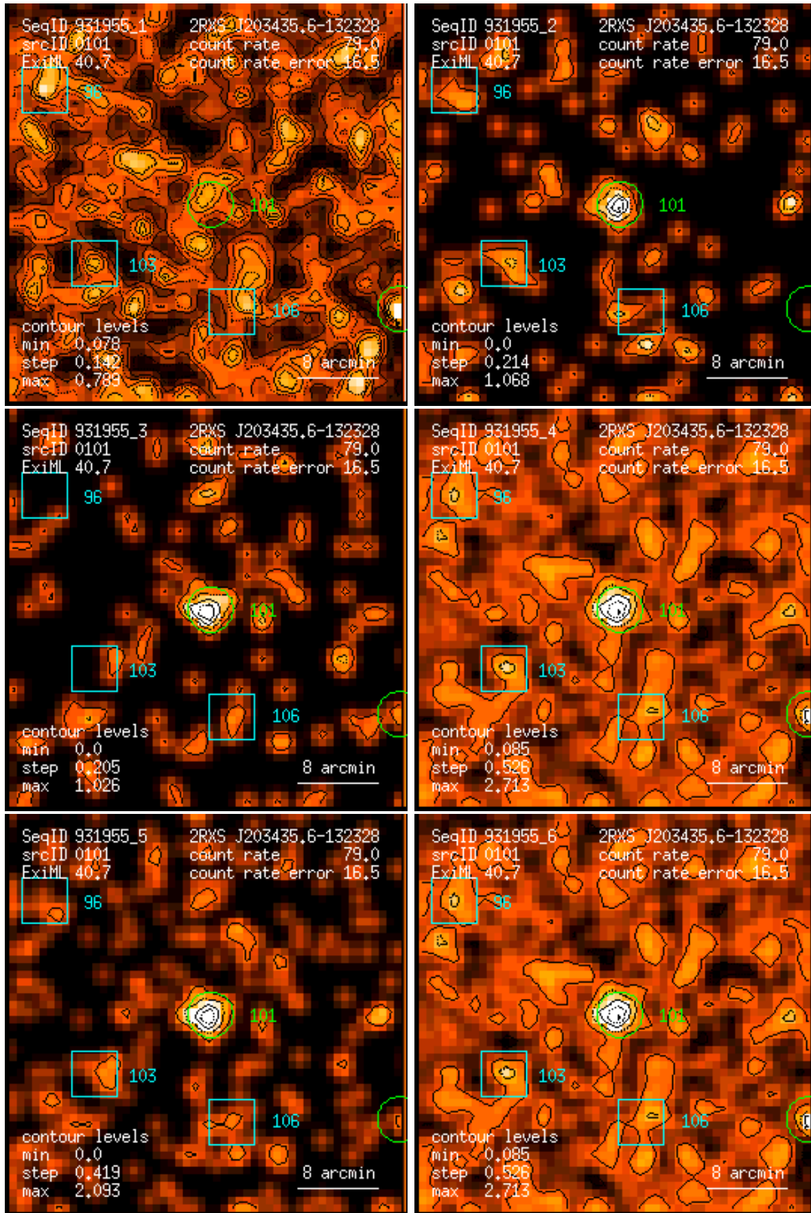
Figure 101: RASS 931955: detection 0101: band rate images, Gaussian filter: (1) PSPC channels 11 – 41, (2) 52 – 90, (3) 91 – 201, (4) 11 – 235, (5) 52 – 201, (6) 11 – 201. Broad band rates in counts/ks. Band rate contour levels in counts/ks/arcmin 2 .
