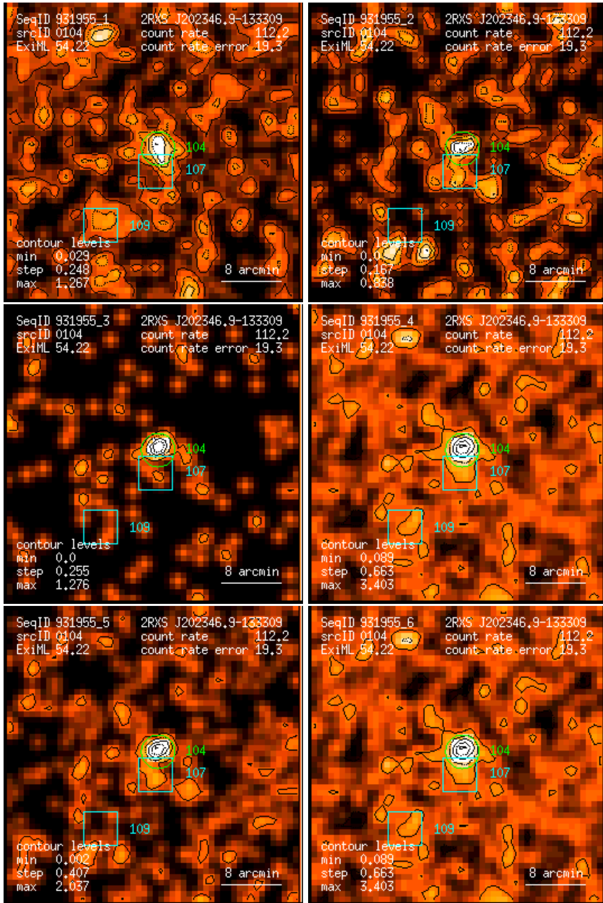
Figure 104: RASS 931955: detection 0104: band rate images, Gaussian filter: (1) PSPC channels 11 – 41, (2) 52 – 90, (3) 91 – 201, (4) 11 – 235, (5) 52 – 201, (6) 11 – 201. Broad band rates in counts/ks. Band rate contour levels in counts/ks/arcmin 2 .
