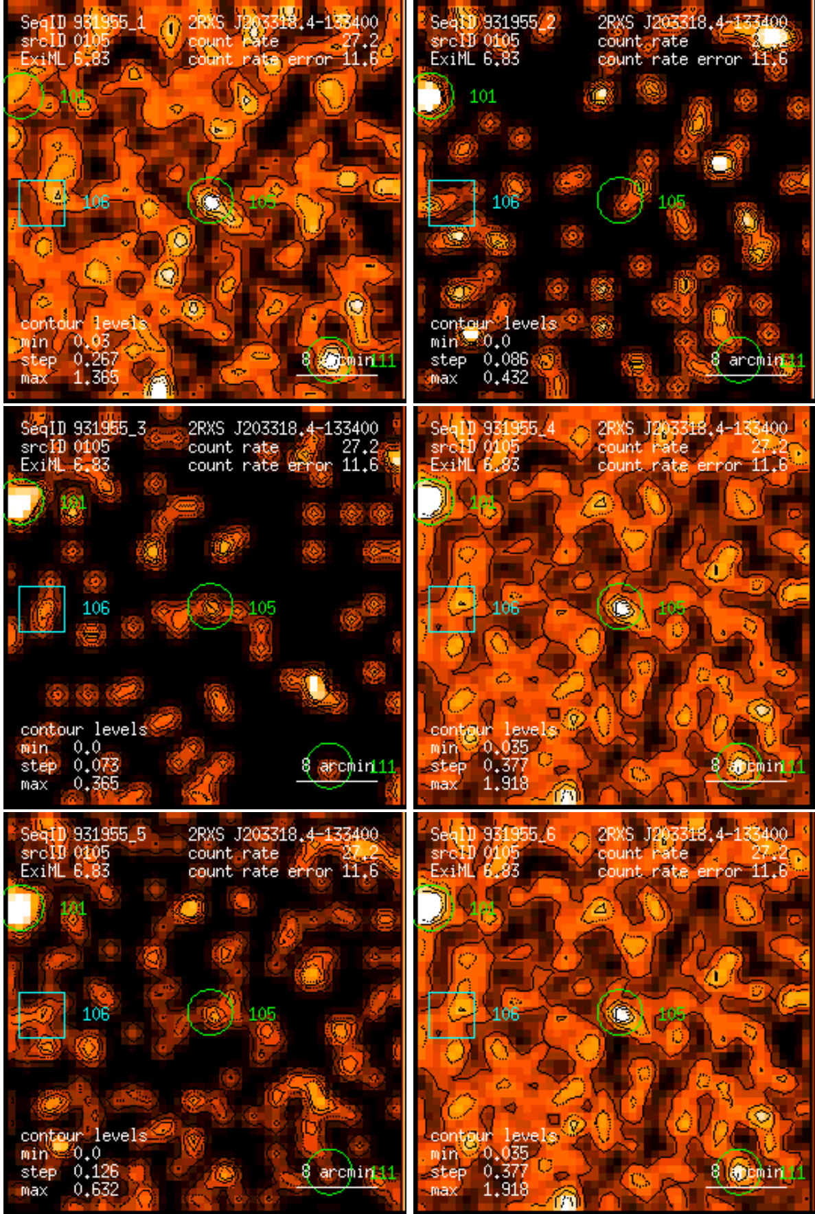
Figure 105: RASS 931955: detection 0105: band rate images, Gaussian filter: (1) PSPC channels 11 – 41, (2) 52 – 90, (3) 91 – 201, (4) 11 – 235, (5) 52 – 201, (6) 11 – 201. Broad band rates in counts/ks. Band rate contour levels in counts/ks/arcmin 2 .
