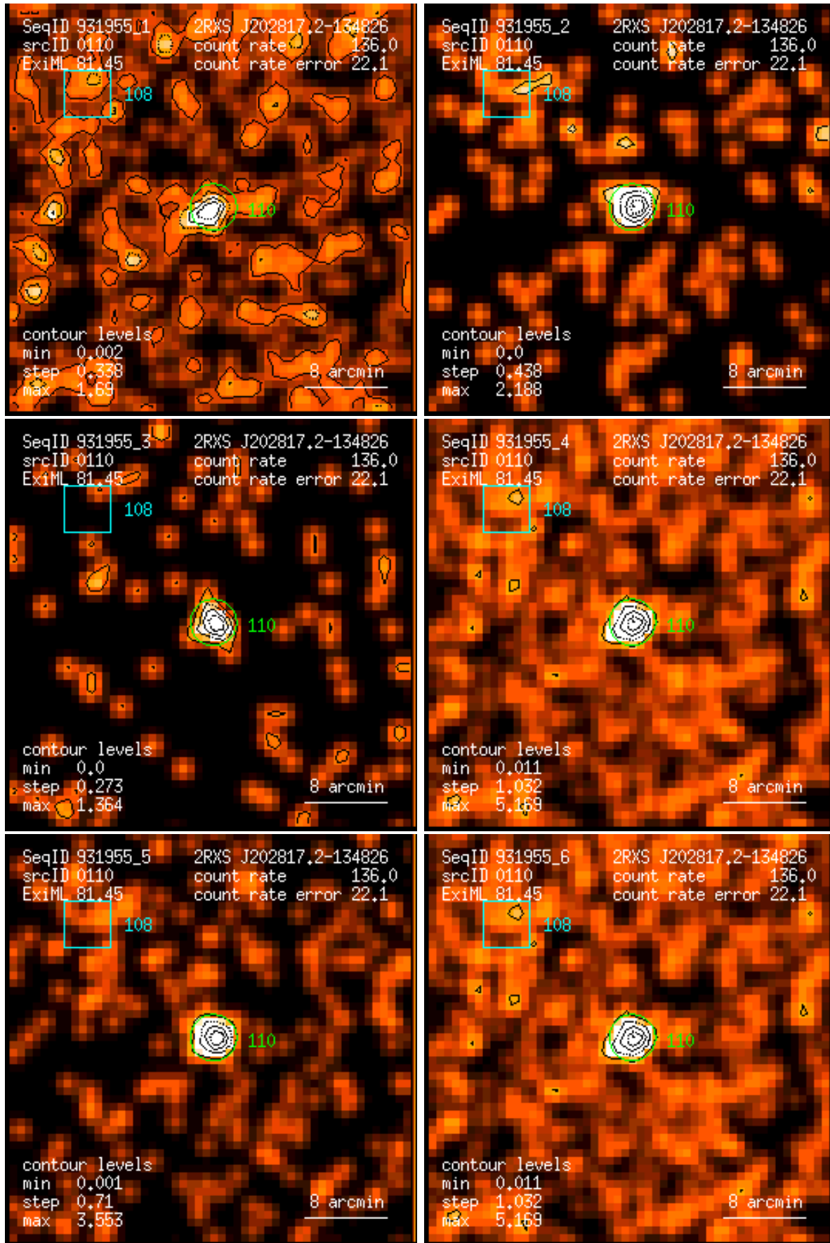
Figure 110: RASS 931955: detection 0110: band rate images, Gaussian filter: (1) PSPC channels 11 – 41, (2) 52 – 90, (3) 91 – 201, (4) 11 – 235, (5) 52 – 201, (6) 11 – 201. Broad band rates in counts/ks. Band rate contour levels in counts/ks/arcmin 2 .
