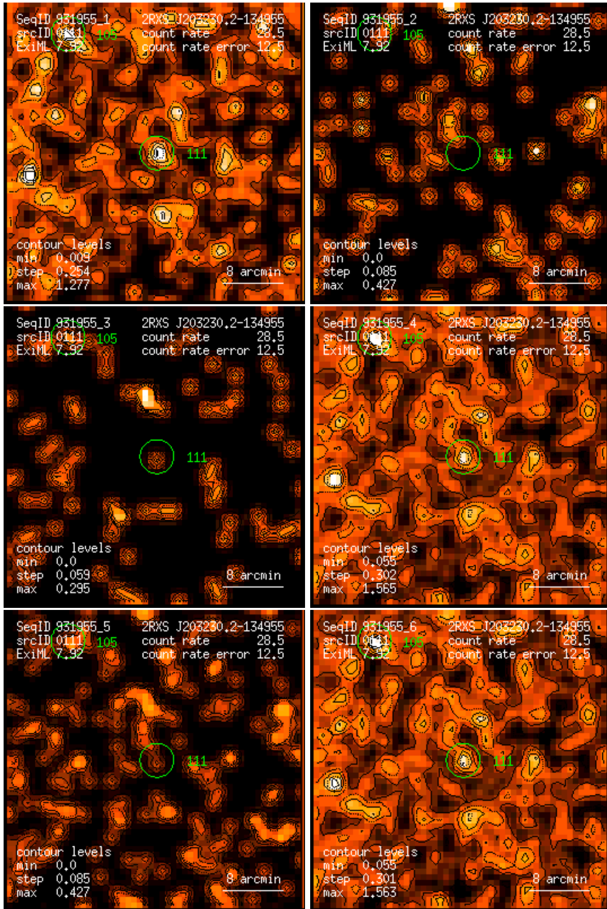
Figure 111: RASS 931955: detection 0111: band rate images, Gaussian filter: (1) PSPC channels 11 – 41, (2) 52 – 90, (3) 91 – 201, (4) 11 – 235, (5) 52 – 201, (6) 11 – 201. Broad band rates in counts/ks. Band rate contour levels in counts/ks/arcmin 2 .
