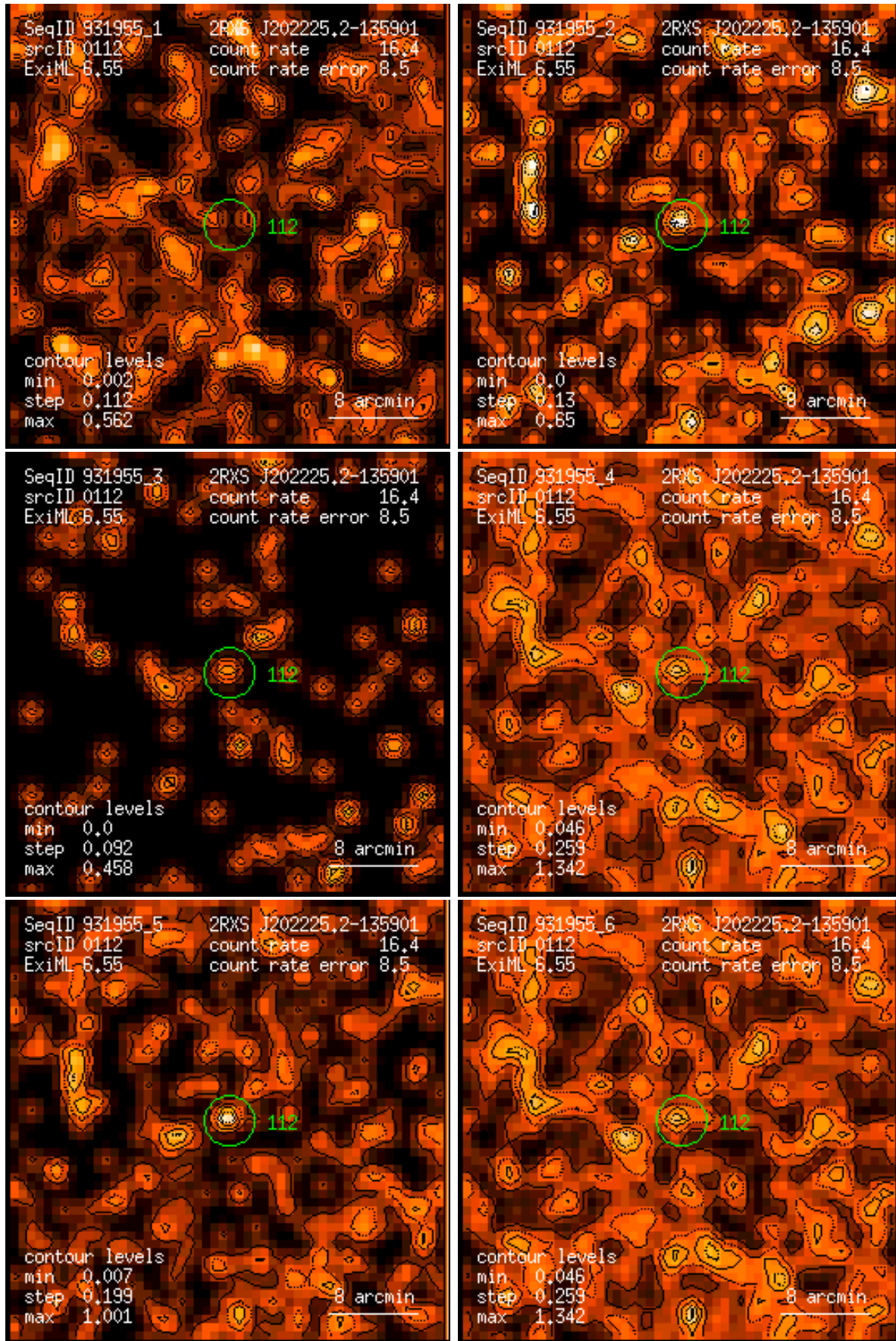
Figure 112: RASS 931955: detection 0112: band rate images, Gaussian filter: (1) PSPC channels 11 – 41, (2) 52 – 90, (3) 91 – 201, (4) 11 – 235, (5) 52 – 201, (6) 11 – 201. Broad band rates in counts/ks. Band rate contour levels in counts/ks/arcmin 2 .
