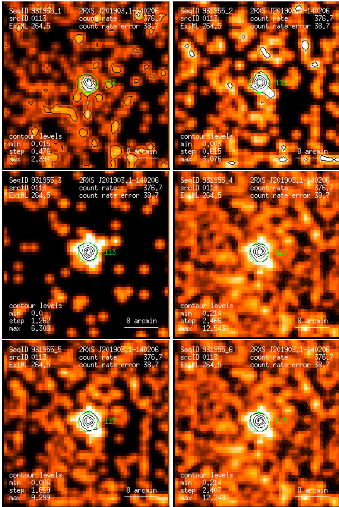
Figure 113: RASS 931955: detection 0113: band rate images, Gaussian filter: (1) PSPC channels 11 – 41, (2) 52 – 90, (3) 91 – 201, (4) 11 – 235, (5) 52 – 201, (6) 11 – 201. Broad band rates in counts/ks. Band rate contour levels in counts/ks/arcmin 2 .
