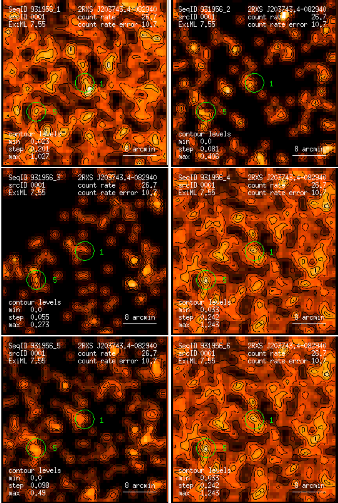
Figure 1: RASS 931956: detection 0001: band rate images, Gaussian filter: (1) PSPC channels 11 – 41, (2) 52 – 90, (3) 91 – 201, (4) 11 – 235, (5) 52 – 201, (6) 11 – 201. Broad band rates in counts/ks. Band rate contour levels in counts/ks/arcmin 2 .
