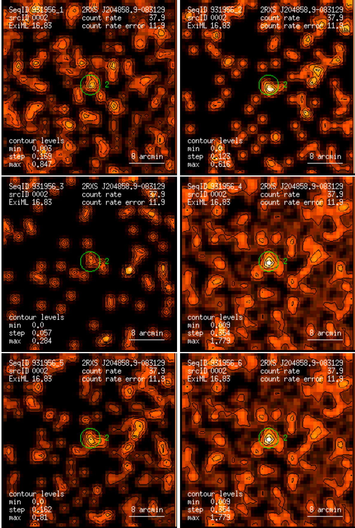
Figure 2: RASS 931956: detection 0002: band rate images, Gaussian filter: (1) PSPC channels 11 – 41, (2) 52 – 90, (3) 91 – 201, (4) 11 – 235, (5) 52 – 201, (6) 11 – 201. Broad band rates in counts/ks. Band rate contour levels in counts/ks/arcmin 2 .
