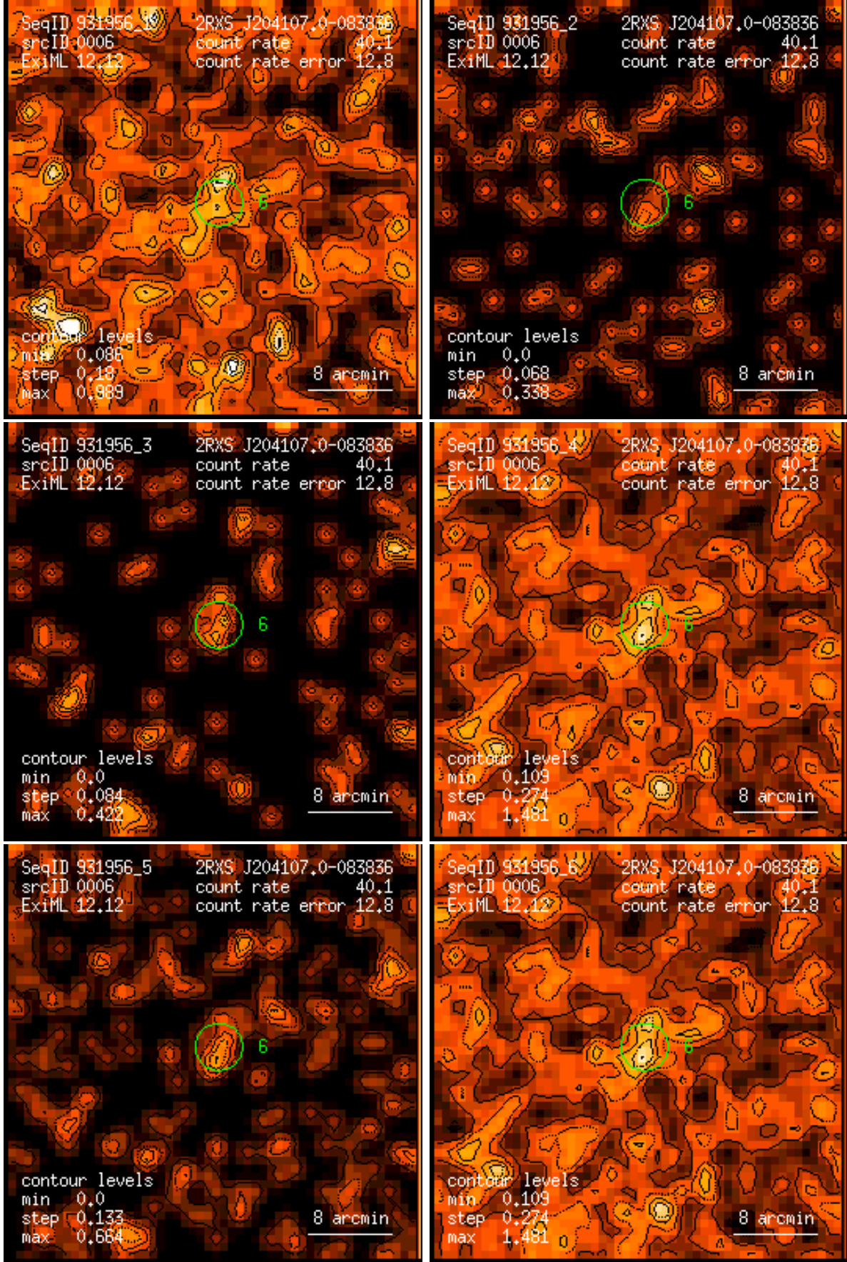
Figure 6: RASS 931956: detection 0006: band rate images, Gaussian filter: (1) PSPC channels 11 – 41, (2) 52 – 90, (3) 91 – 201, (4) 11 – 235, (5) 52 – 201, (6) 11 – 201. Broad band rates in counts/ks. Band rate contour levels in counts/ks/arcmin 2 .
