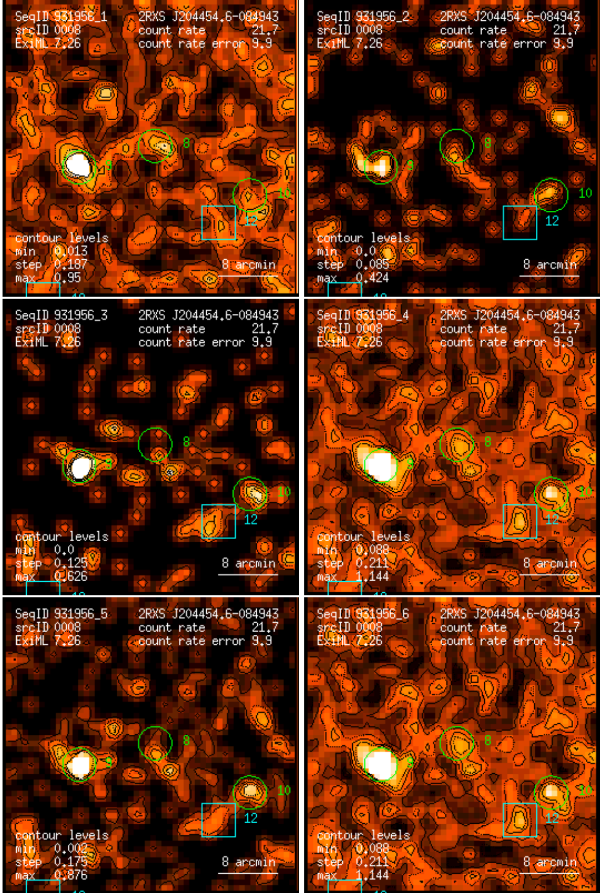
Figure 8: RASS 931956: detection 0008: band rate images, Gaussian filter: (1) PSPC channels 11 – 41, (2) 52 – 90, (3) 91 – 201, (4) 11 – 235, (5) 52 – 201, (6) 11 – 201. Broad band rates in counts/ks. Band rate contour levels in counts/ks/arcmin 2 .
