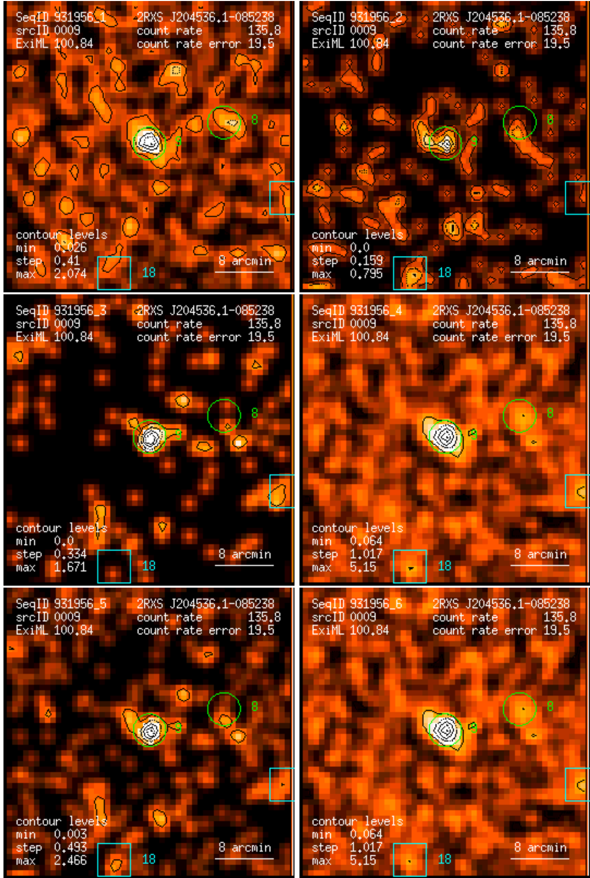
Figure 9: RASS 931956: detection 0009: band rate images, Gaussian filter: (1) PSPC channels 11 – 41, (2) 52 – 90, (3) 91 – 201, (4) 11 – 235, (5) 52 – 201, (6) 11 – 201. Broad band rates in counts/ks. Band rate contour levels in counts/ks/arcmin 2 .
