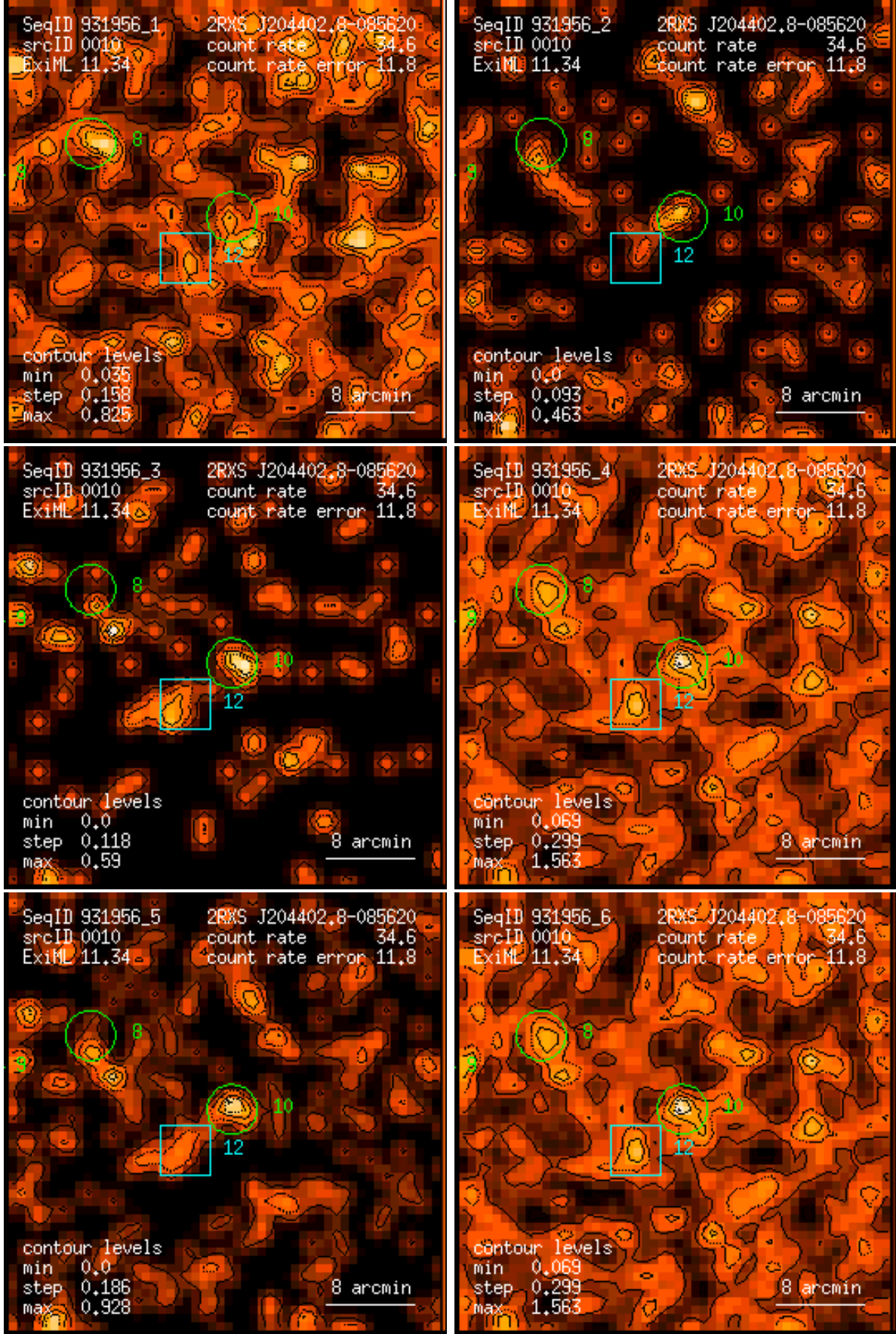
Figure 10: RASS 931956: detection 0010: band rate images, Gaussian filter: (1) PSPC channels 11 – 41, (2) 52 – 90, (3) 91 – 201, (4) 11 – 235, (5) 52 – 201, (6) 11 – 201. Broad band rates in counts/ks. Band rate contour levels in counts/ks/arcmin 2 .
