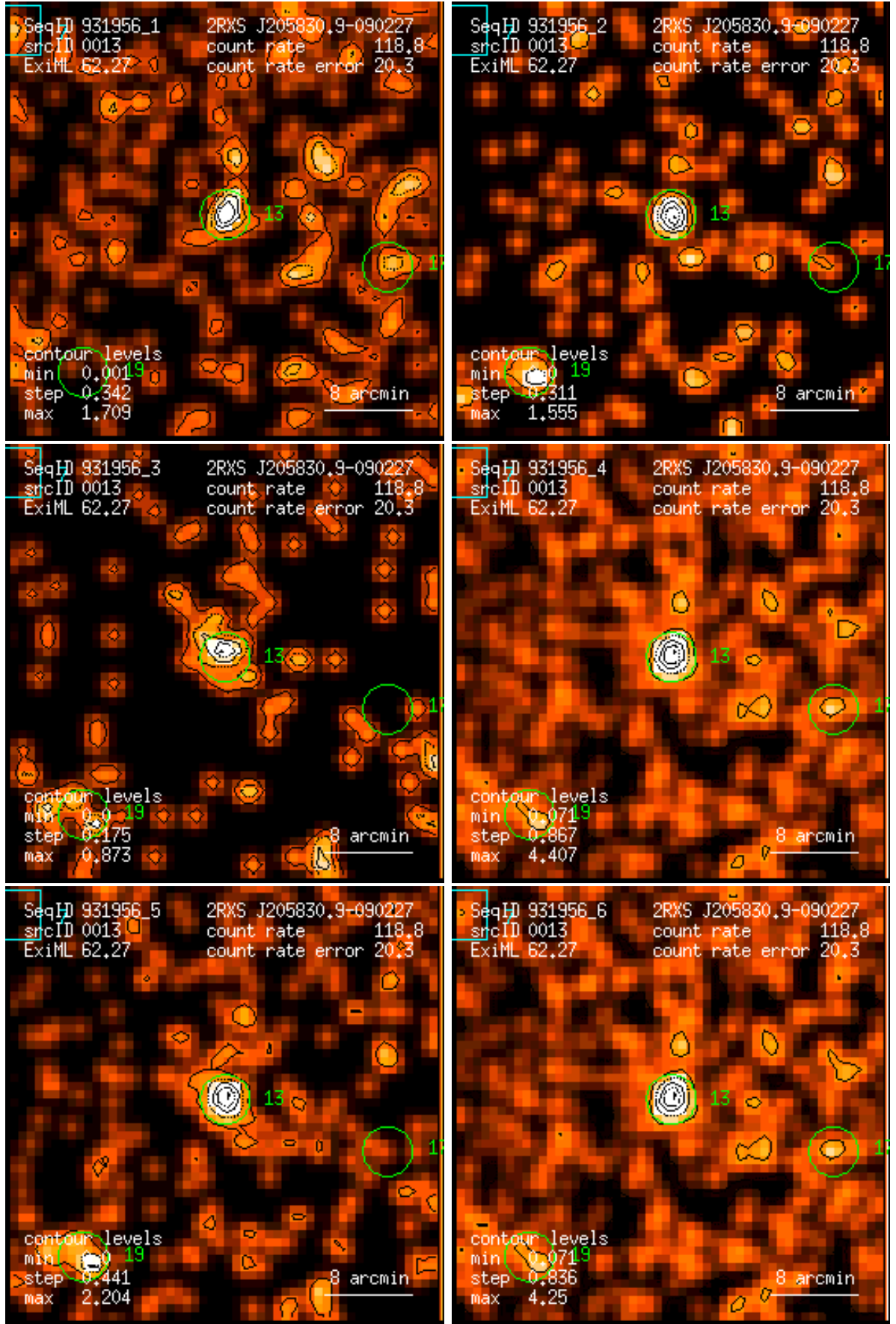
Figure 13: RASS 931956: detection 0013: band rate images, Gaussian filter: (1) PSPC channels 11 – 41, (2) 52 – 90, (3) 91 – 201, (4) 11 – 235, (5) 52 – 201, (6) 11 – 201. Broad band rates in counts/ks. Band rate contour levels in counts/ks/arcmin 2 .
