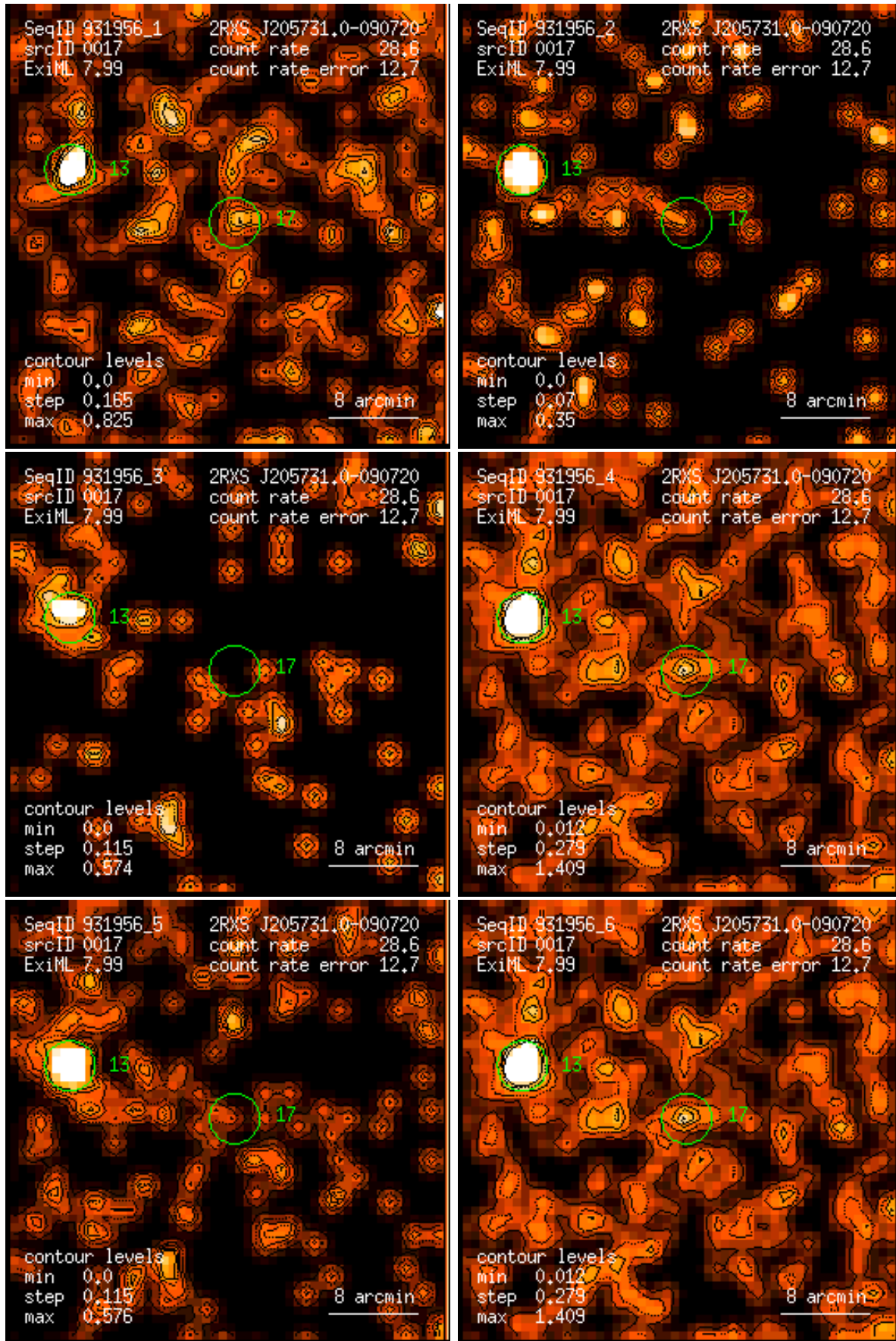
Figure 17: RASS 931956: detection 0017: band rate images, Gaussian filter: (1) PSPC channels 11 – 41, (2) 52 – 90, (3) 91 – 201, (4) 11 – 235, (5) 52 – 201, (6) 11 – 201. Broad band rates in counts/ks. Band rate contour levels in counts/ks/arcmin 2 .
