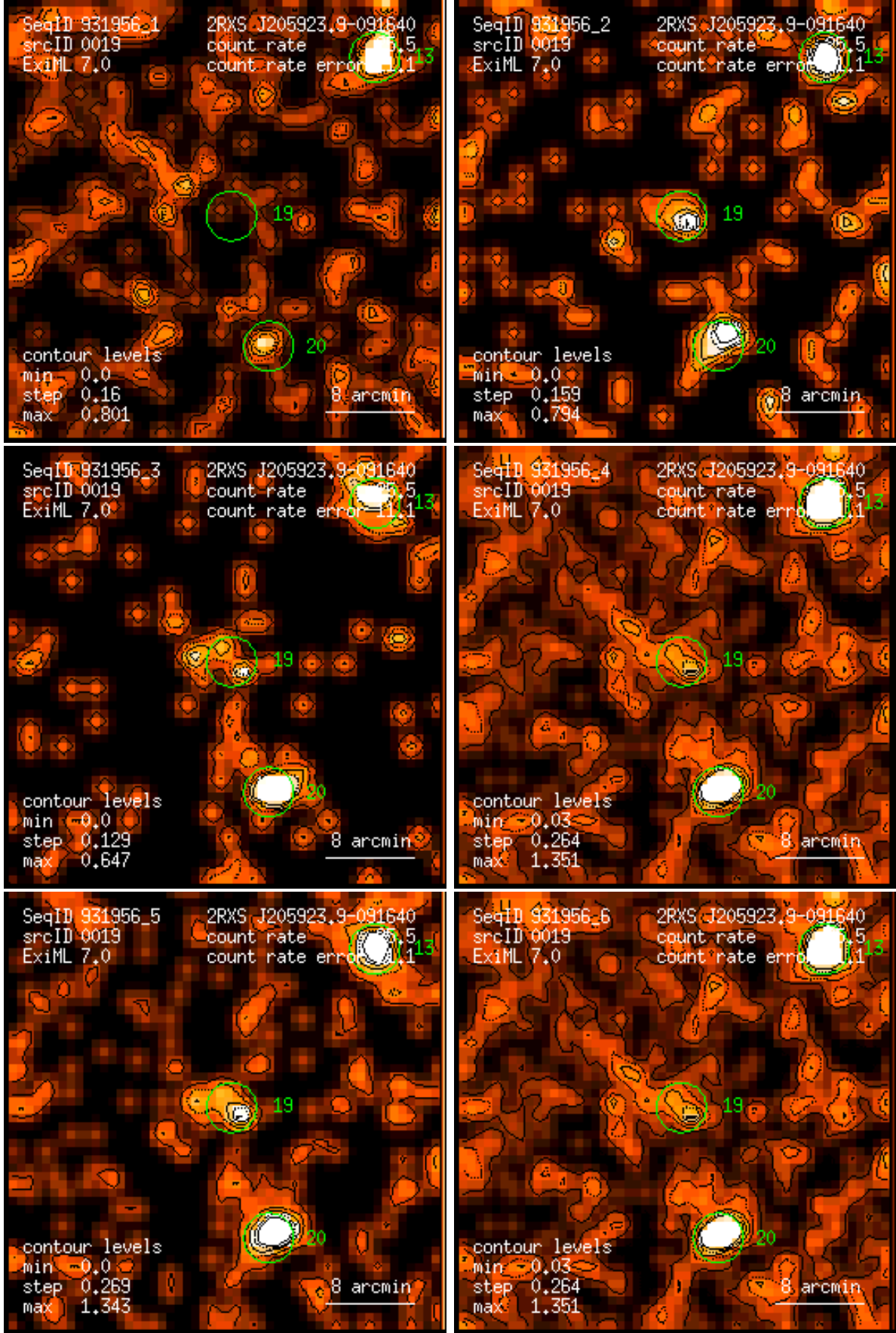
Figure 19: RASS 931956: detection 0019: band rate images, Gaussian filter: (1) PSPC channels 11 – 41, (2) 52 – 90, (3) 91 – 201, (4) 11 – 235, (5) 52 – 201, (6) 11 – 201. Broad band rates in counts/ks. Band rate contour levels in counts/ks/arcmin 2 .
