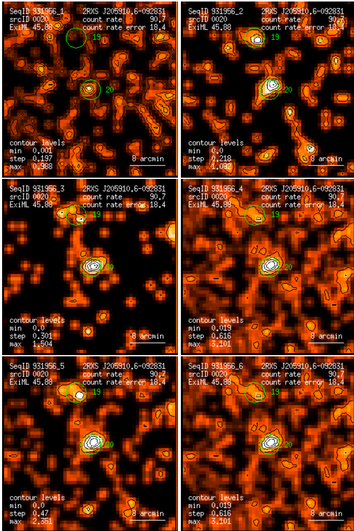
Figure 20: RASS 931956: detection 0020: band rate images, Gaussian filter: (1) PSPC channels 11 – 41, (2) 52 – 90, (3) 91 – 201, (4) 11 – 235, (5) 52 – 201, (6) 11 – 201. Broad band rates in counts/ks. Band rate contour levels in counts/ks/arcmin 2 .
