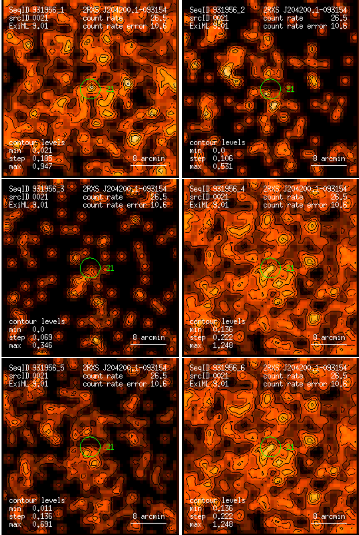
Figure 21: RASS 931956: detection 0021: band rate images, Gaussian filter: (1) PSPC channels 11 – 41, (2) 52 – 90, (3) 91 – 201, (4) 11 – 235, (5) 52 – 201, (6) 11 – 201. Broad band rates in counts/ks. Band rate contour levels in counts/ks/arcmin 2 .
