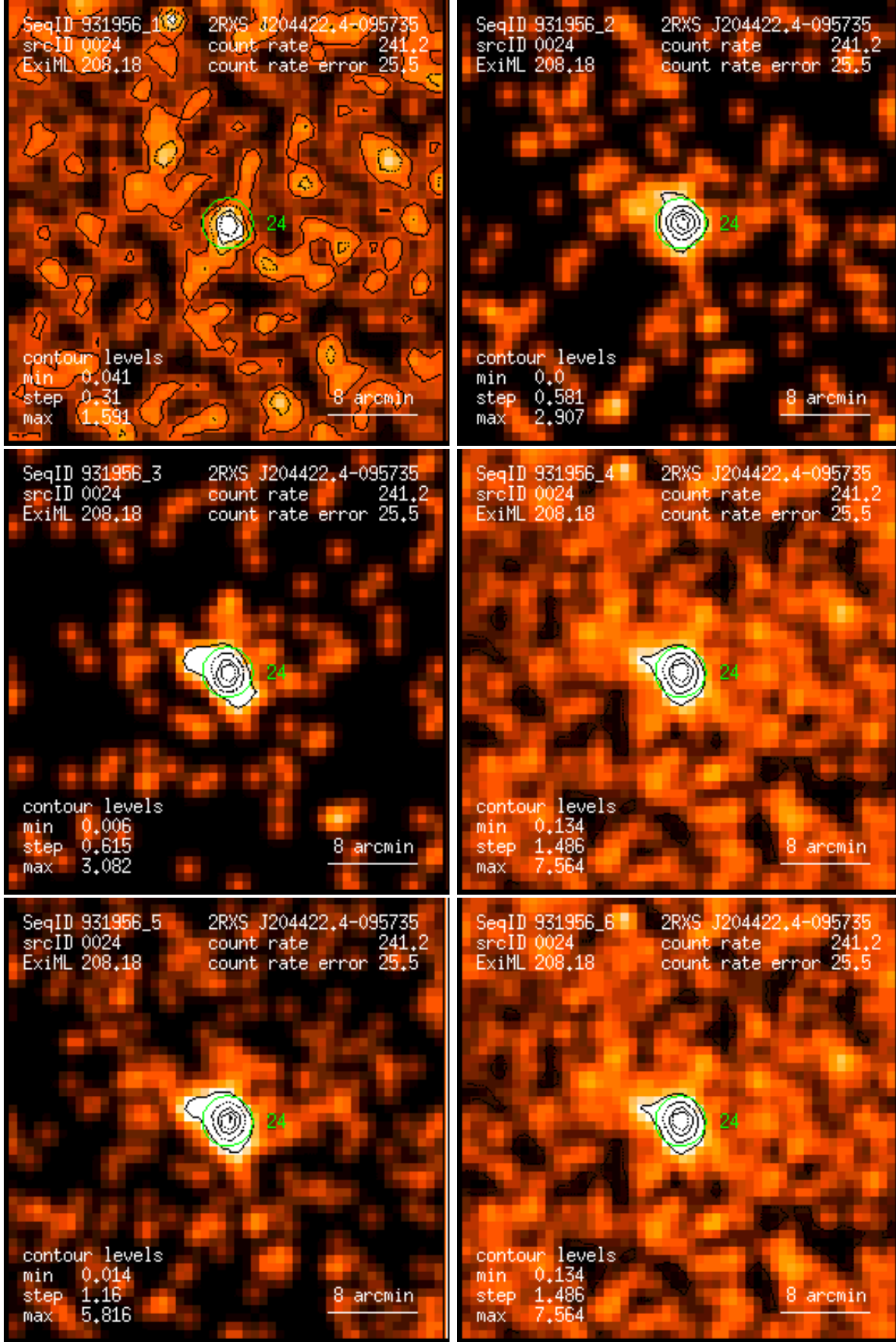
Figure 24: RASS 931956: detection 0024: band rate images, Gaussian filter: (1) PSPC channels 11 – 41, (2) 52 – 90, (3) 91 – 201, (4) 11 – 235, (5) 52 – 201, (6) 11 – 201. Broad band rates in counts/ks. Band rate contour levels in counts/ks/arcmin 2 .
