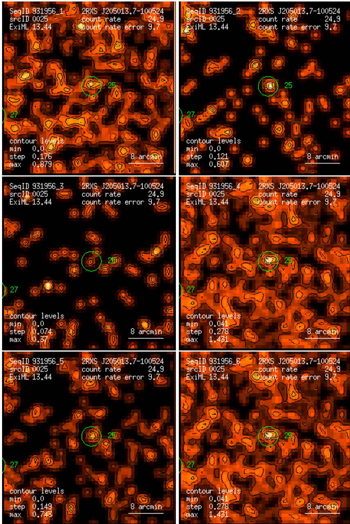
Figure 25: RASS 931956: detection 0025: band rate images, Gaussian filter: (1) PSPC channels 11 – 41, (2) 52 – 90, (3) 91 – 201, (4) 11 – 235, (5) 52 – 201, (6) 11 – 201. Broad band rates in counts/ks. Band rate contour levels in counts/ks/arcmin 2 .
