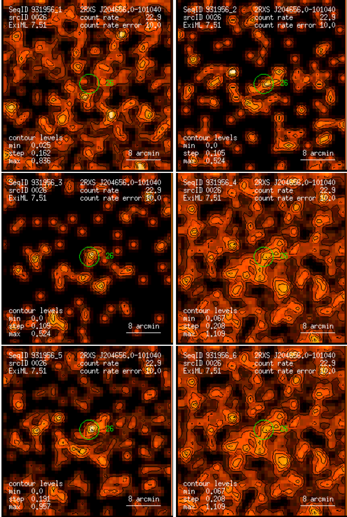
Figure 26: RASS 931956: detection 0026: band rate images, Gaussian filter: (1) PSPC channels 11 – 41, (2) 52 – 90, (3) 91 – 201, (4) 11 – 235, (5) 52 – 201, (6) 11 – 201. Broad band rates in counts/ks. Band rate contour levels in counts/ks/arcmin 2 .
