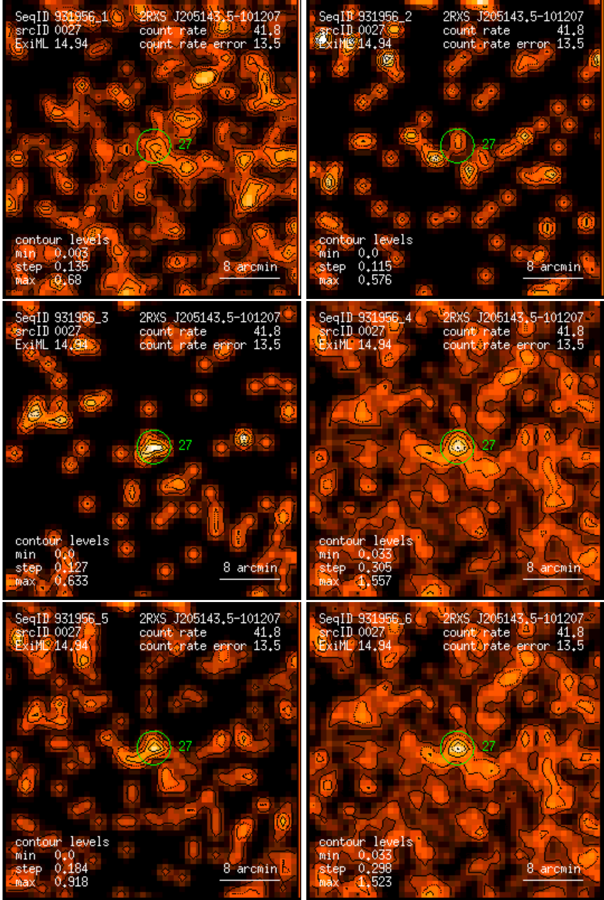
Figure 27: RASS 931956: detection 0027: band rate images, Gaussian filter: (1) PSPC channels 11 – 41, (2) 52 – 90, (3) 91 – 201, (4) 11 – 235, (5) 52 – 201, (6) 11 – 201. Broad band rates in counts/ks. Band rate contour levels in counts/ks/arcmin 2 .
