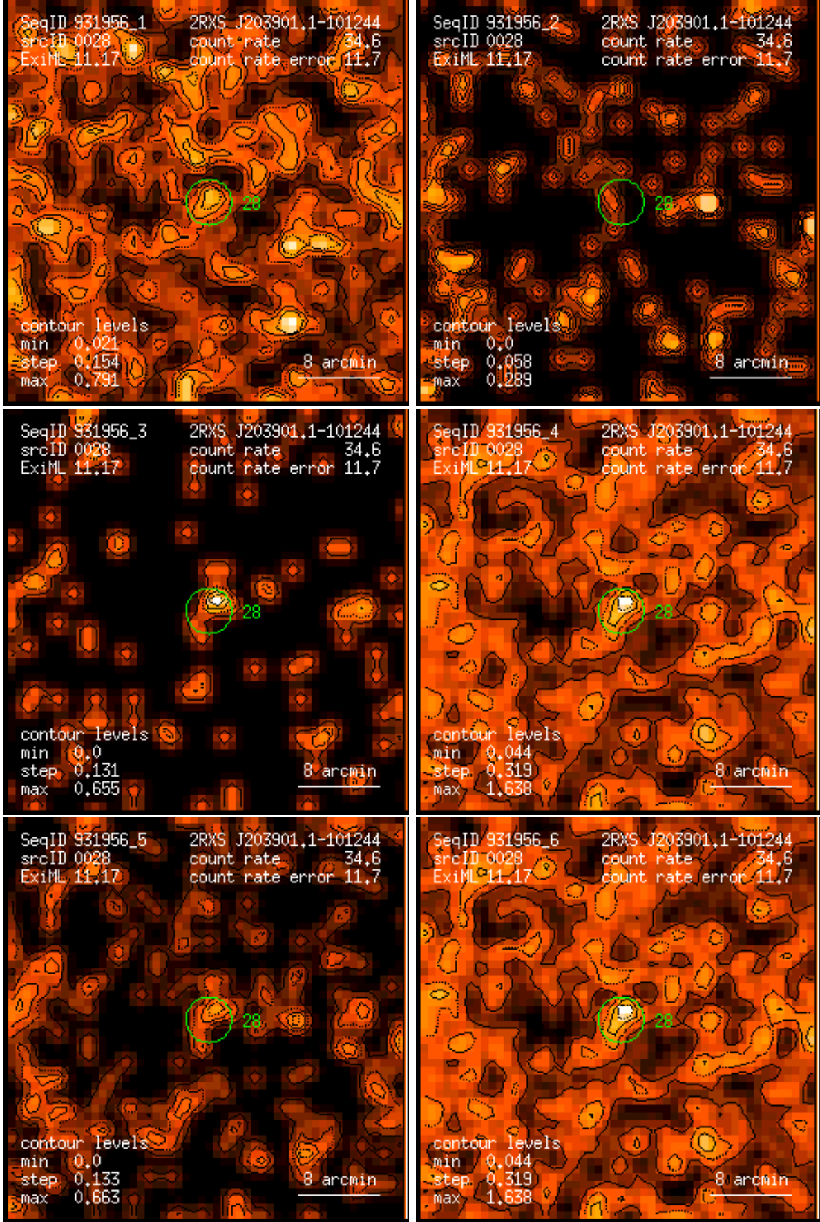
Figure 28: RASS 931956: detection 0028: band rate images, Gaussian filter: (1) PSPC channels 11 – 41, (2) 52 – 90, (3) 91 – 201, (4) 11 – 235, (5) 52 – 201, (6) 11 – 201. Broad band rates in counts/ks. Band rate contour levels in counts/ks/arcmin 2 .
