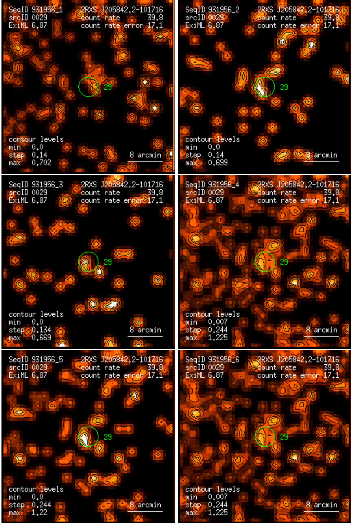
Figure 29: RASS 931956: detection 0029: band rate images, Gaussian filter: (1) PSPC channels 11 – 41, (2) 52 – 90, (3) 91 – 201, (4) 11 – 235, (5) 52 – 201, (6) 11 – 201. Broad band rates in counts/ks. Band rate contour levels in counts/ks/arcmin 2 .
