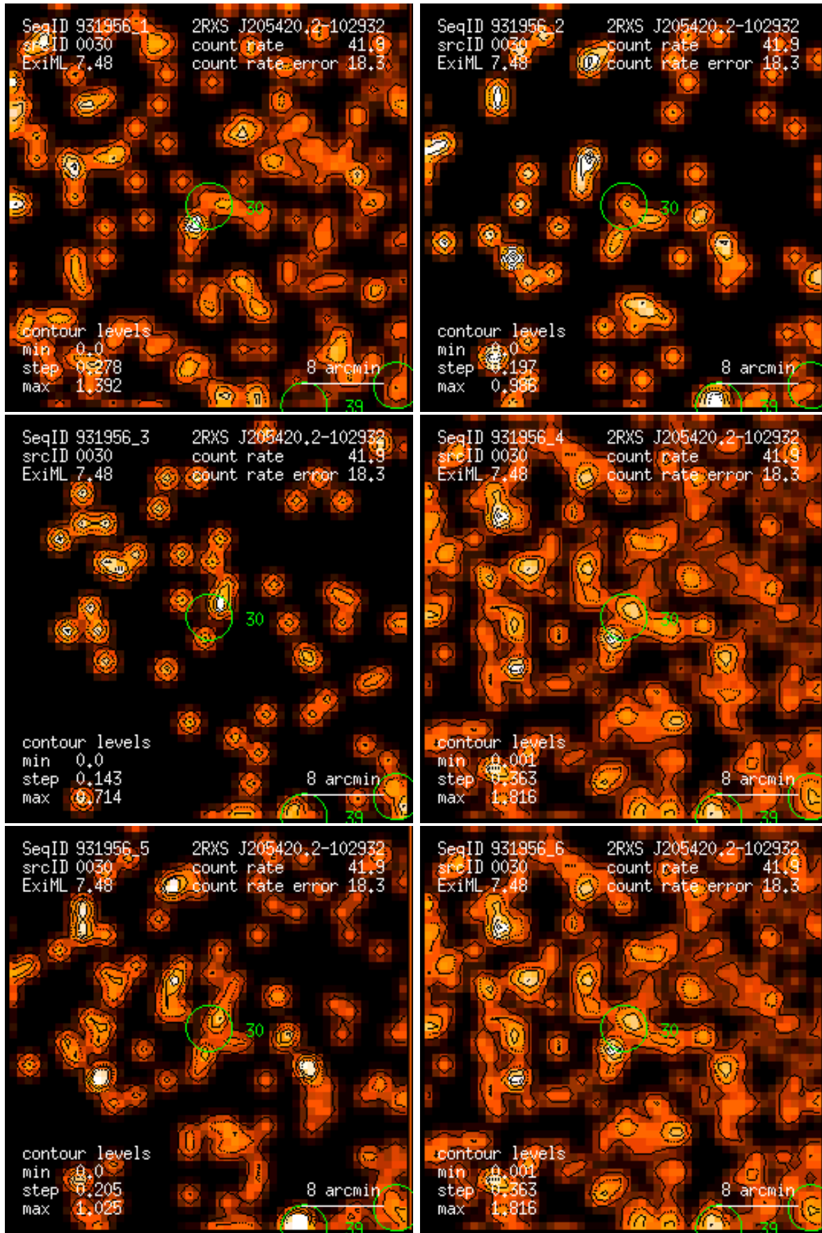
Figure 30: RASS 931956: detection 0030: band rate images, Gaussian filter: (1) PSPC channels 11 – 41, (2) 52 – 90, (3) 91 – 201, (4) 11 – 235, (5) 52 – 201, (6) 11 – 201. Broad band rates in counts/ks. Band rate contour levels in counts/ks/arcmin 2 .
