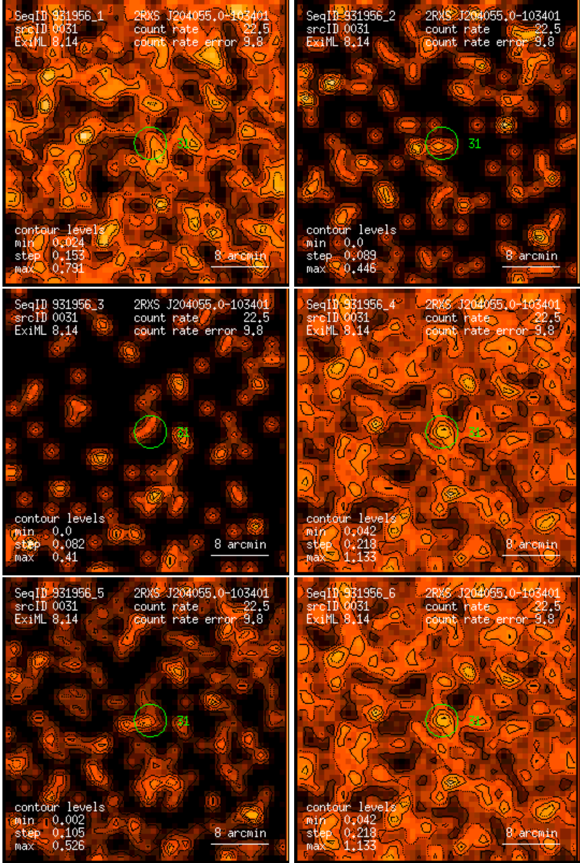
Figure 31: RASS 931956: detection 0031: band rate images, Gaussian filter: (1) PSPC channels 11 – 41, (2) 52 – 90, (3) 91 – 201, (4) 11 – 235, (5) 52 – 201, (6) 11 – 201. Broad band rates in counts/ks. Band rate contour levels in counts/ks/arcmin 2 .
