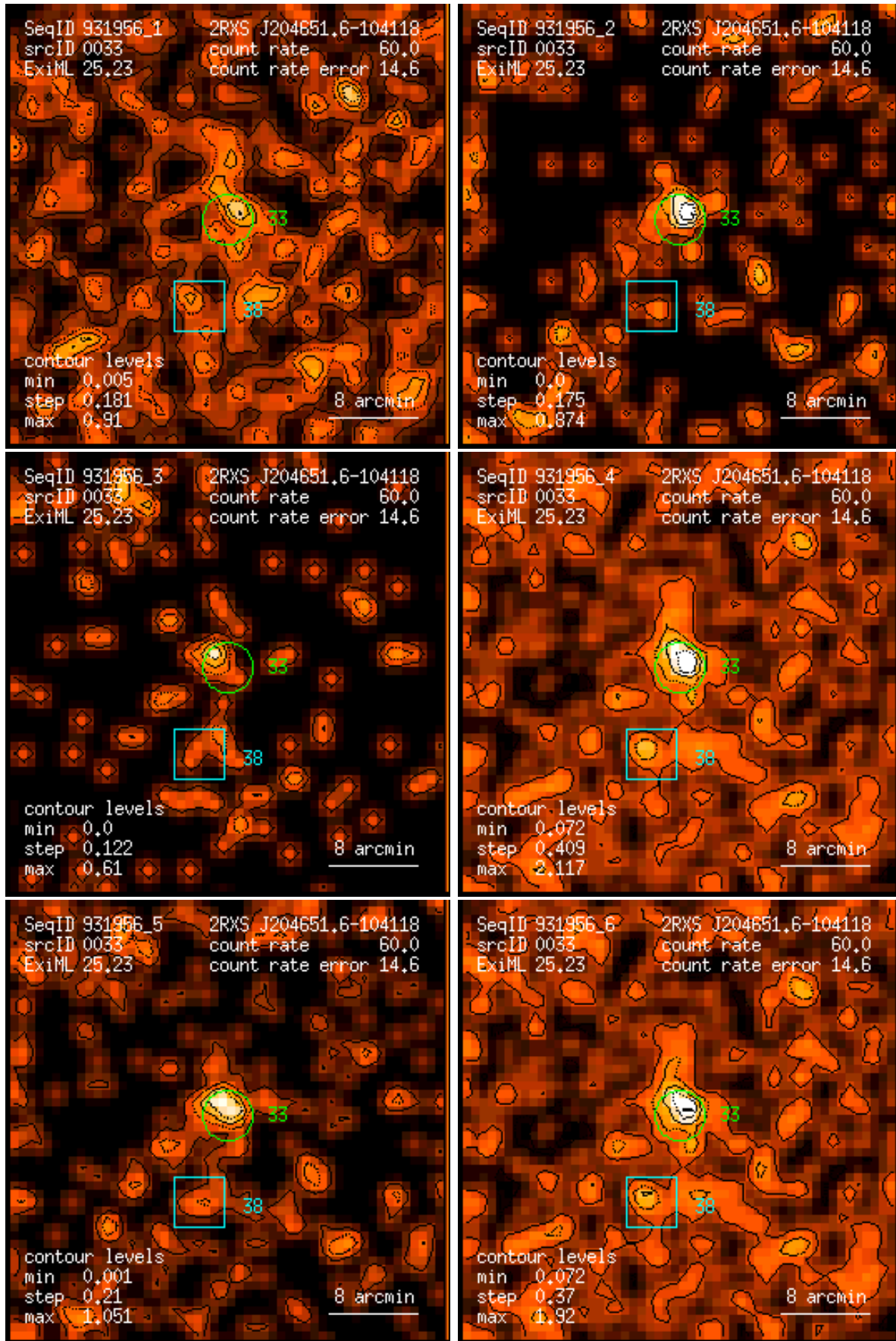
Figure 33: RASS 931956: detection 0033: band rate images, Gaussian filter: (1) PSPC channels 11 – 41, (2) 52 – 90, (3) 91 – 201, (4) 11 – 235, (5) 52 – 201, (6) 11 – 201. Broad band rates in counts/ks. Band rate contour levels in counts/ks/arcmin 2 .
