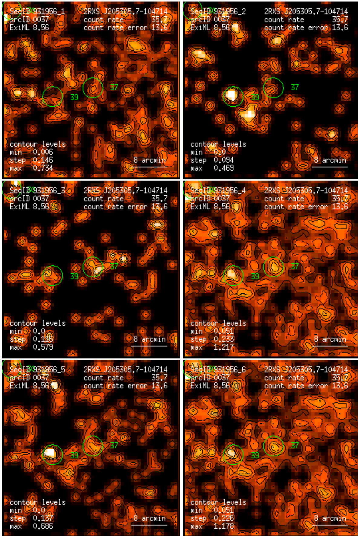
Figure 37: RASS 931956: detection 0037: band rate images, Gaussian filter: (1) PSPC channels 11 – 41, (2) 52 – 90, (3) 91 – 201, (4) 11 – 235, (5) 52 – 201, (6) 11 – 201. Broad band rates in counts/ks. Band rate contour levels in counts/ks/arcmin 2 .
