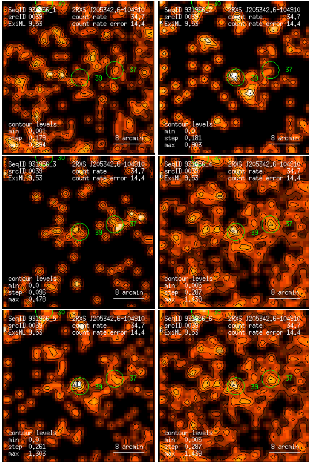
Figure 39: RASS 931956: detection 0039: band rate images, Gaussian filter: (1) PSPC channels 11 – 41, (2) 52 – 90, (3) 91 – 201, (4) 11 – 235, (5) 52 – 201, (6) 11 – 201. Broad band rates in counts/ks. Band rate contour levels in counts/ks/arcmin 2 .
