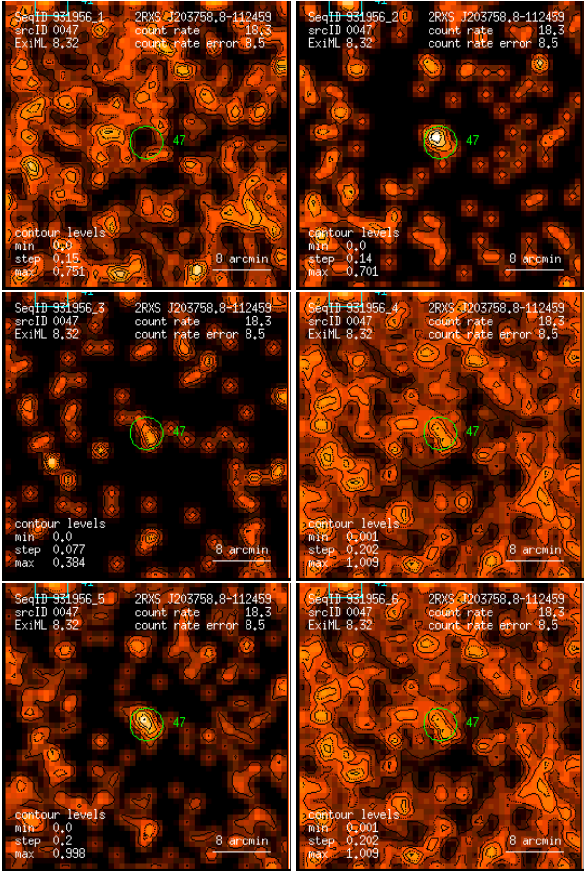
Figure 47: RASS 931956: detection 0047: band rate images, Gaussian filter: (1) PSPC channels 11 – 41, (2) 52 – 90, (3) 91 – 201, (4) 11 – 235, (5) 52 – 201, (6) 11 – 201. Broad band rates in counts/ks. Band rate contour levels in counts/ks/arcmin 2 .
