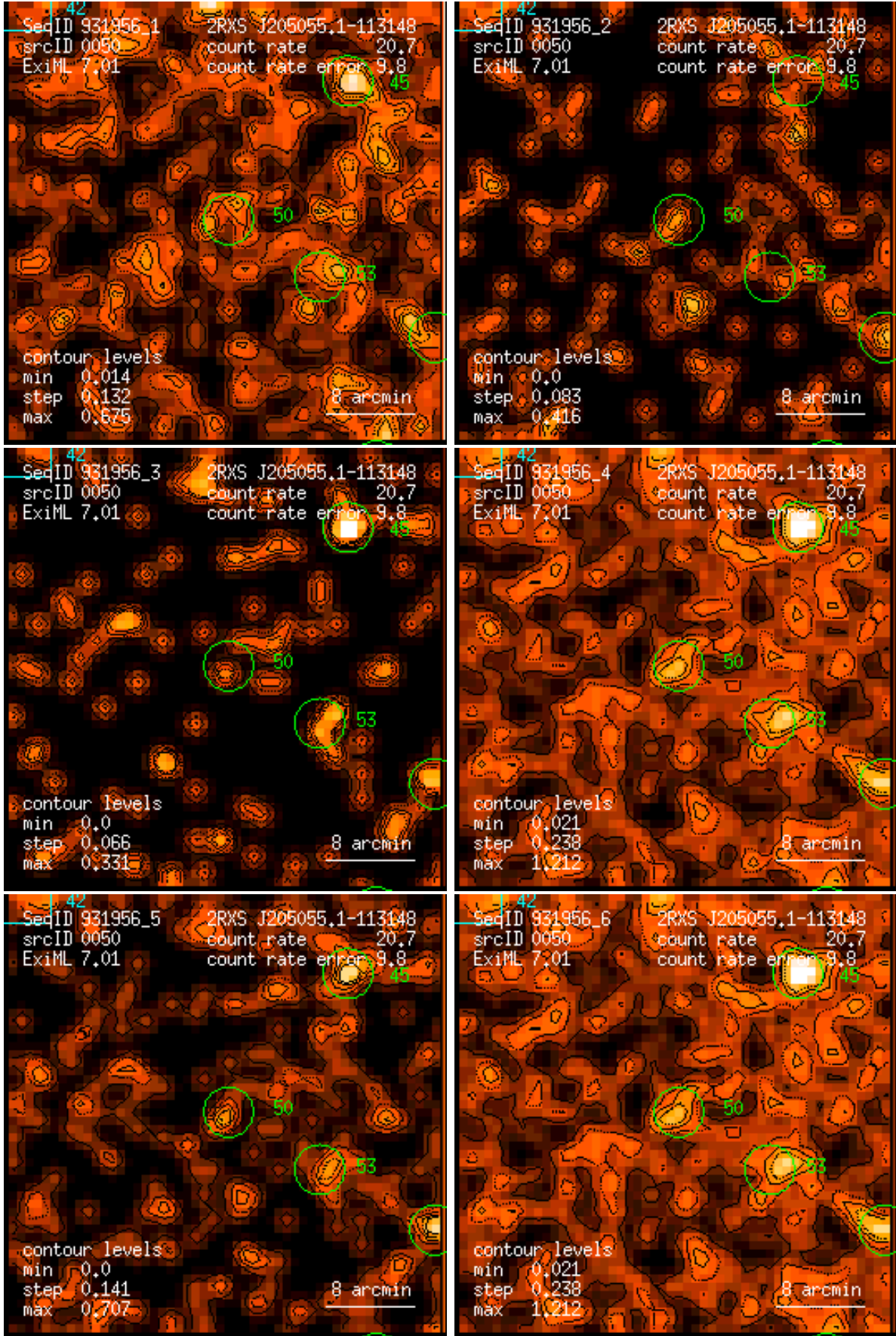
Figure 50: RASS 931956: detection 0050: band rate images, Gaussian filter: (1) PSPC channels 11 – 41, (2) 52 – 90, (3) 91 – 201, (4) 11 – 235, (5) 52 – 201, (6) 11 – 201. Broad band rates in counts/ks. Band rate contour levels in counts/ks/arcmin 2 .
