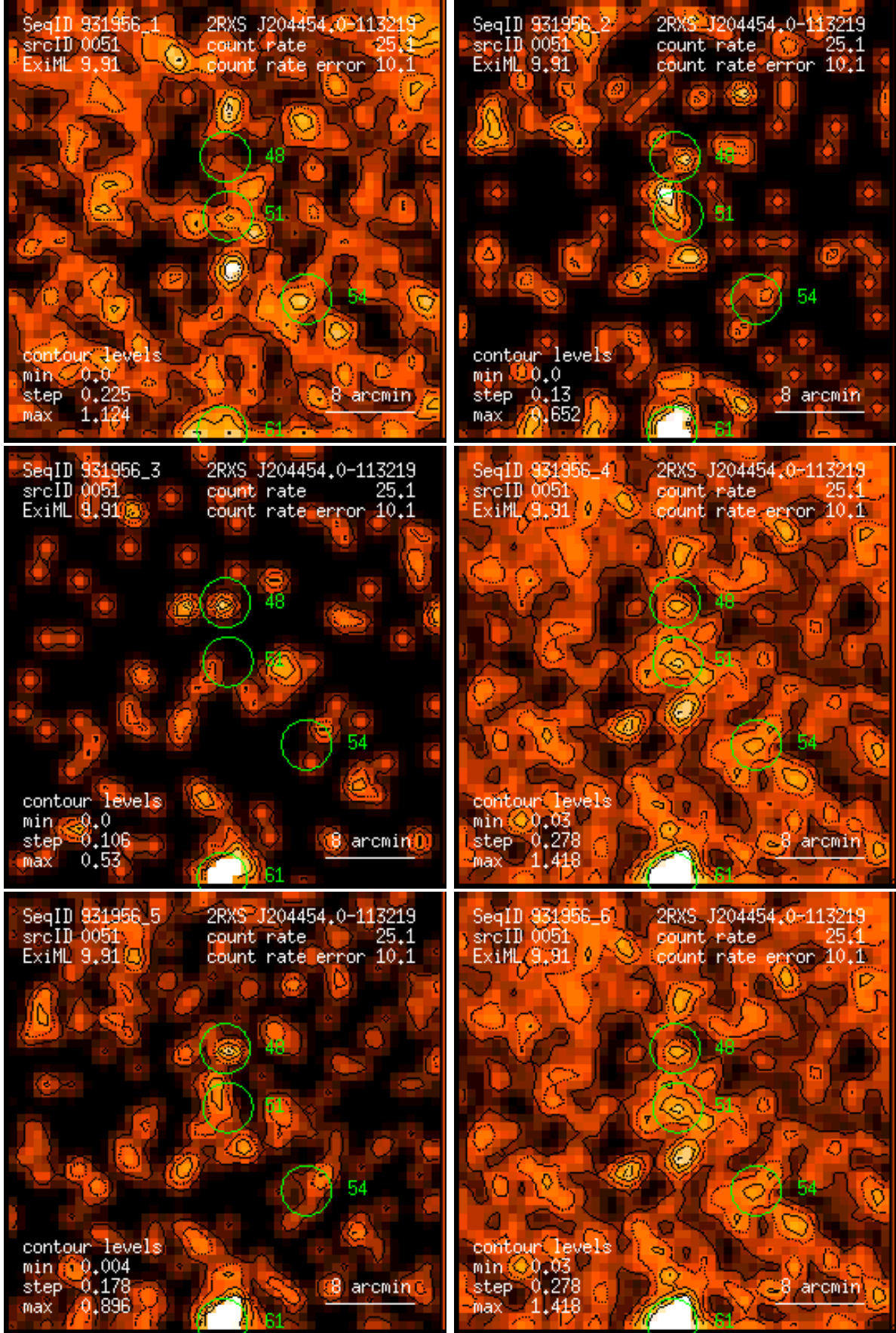
Figure 51: RASS 931956: detection 0051: band rate images, Gaussian filter: (1) PSPC channels 11 – 41, (2) 52 – 90, (3) 91 – 201, (4) 11 – 235, (5) 52 – 201, (6) 11 – 201. Broad band rates in counts/ks. Band rate contour levels in counts/ks/arcmin 2 .
