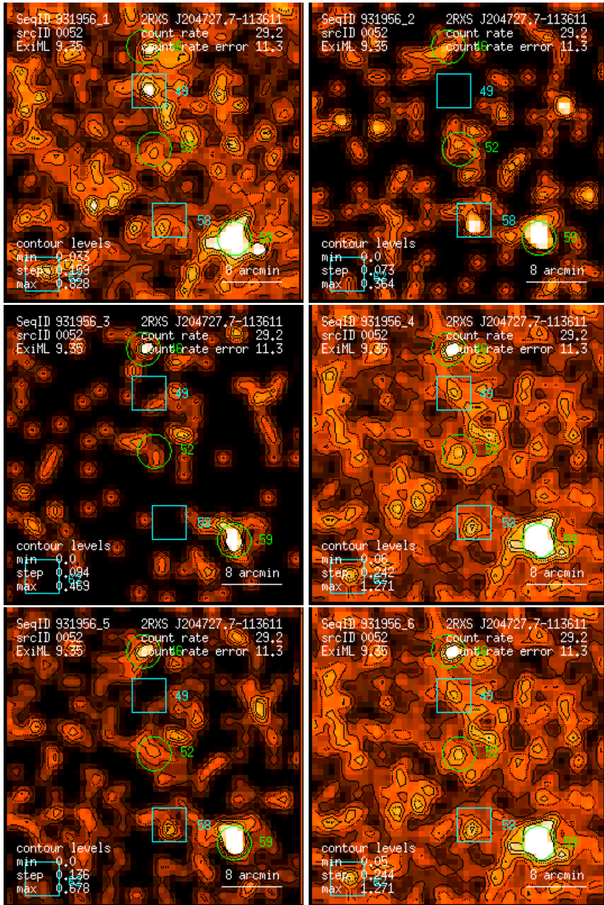
Figure 52: RASS 931956: detection 0052: band rate images, Gaussian filter: (1) PSPC channels 11 – 41, (2) 52 – 90, (3) 91 – 201, (4) 11 – 235, (5) 52 – 201, (6) 11 – 201. Broad band rates in counts/ks. Band rate contour levels in counts/ks/arcmin 2 .
