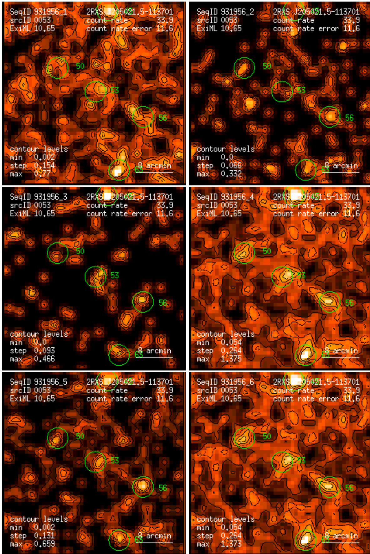
Figure 53: RASS 931956: detection 0053: band rate images, Gaussian filter: (1) PSPC channels 11 – 41, (2) 52 – 90, (3) 91 – 201, (4) 11 – 235, (5) 52 – 201, (6) 11 – 201. Broad band rates in counts/ks. Band rate contour levels in counts/ks/arcmin 2 .
