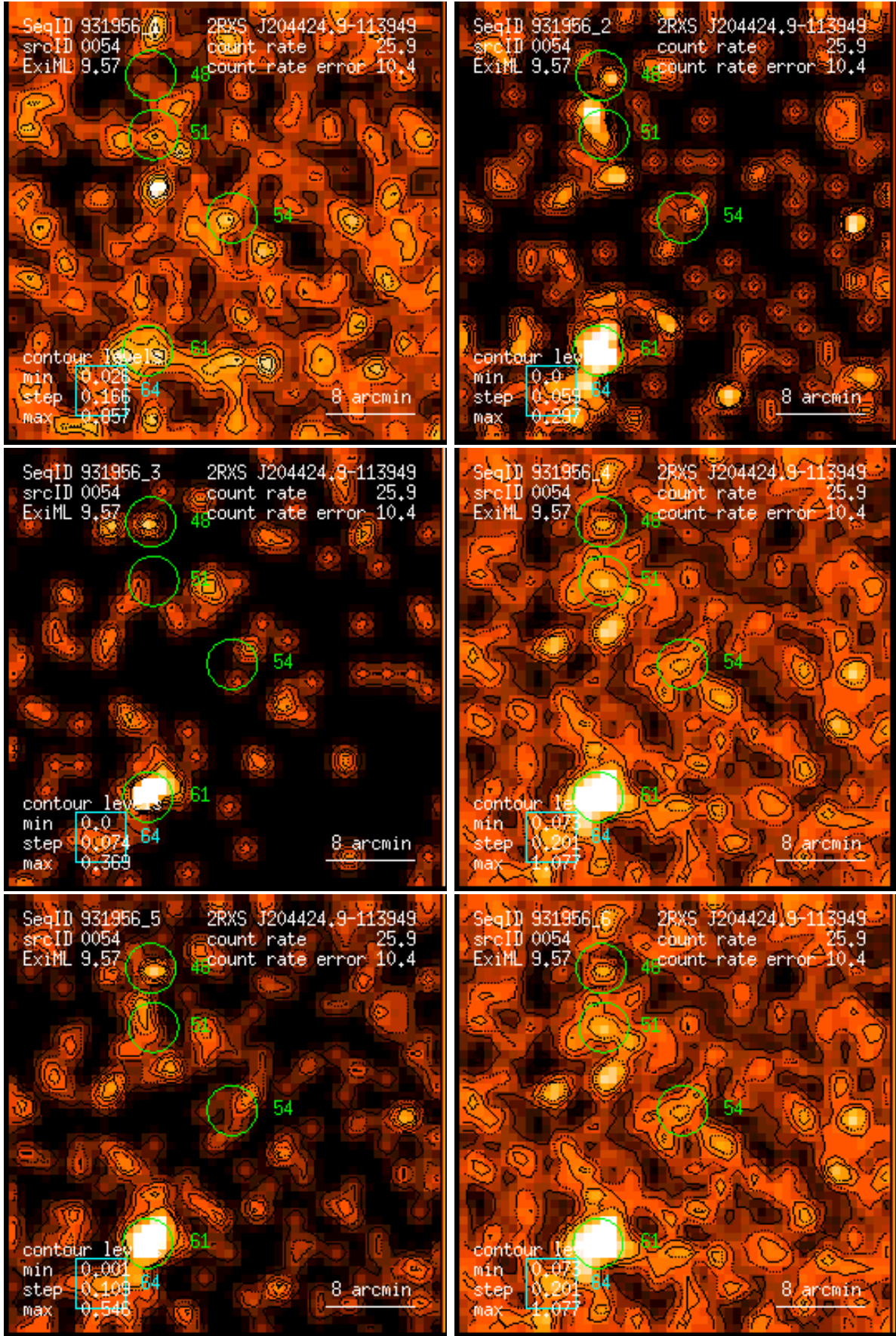
Figure 54: RASS 931956: detection 0054: band rate images, Gaussian filter: (1) PSPC channels 11 – 41, (2) 52 – 90, (3) 91 – 201, (4) 11 – 235, (5) 52 – 201, (6) 11 – 201. Broad band rates in counts/ks. Band rate contour levels in counts/ks/arcmin 2 .
