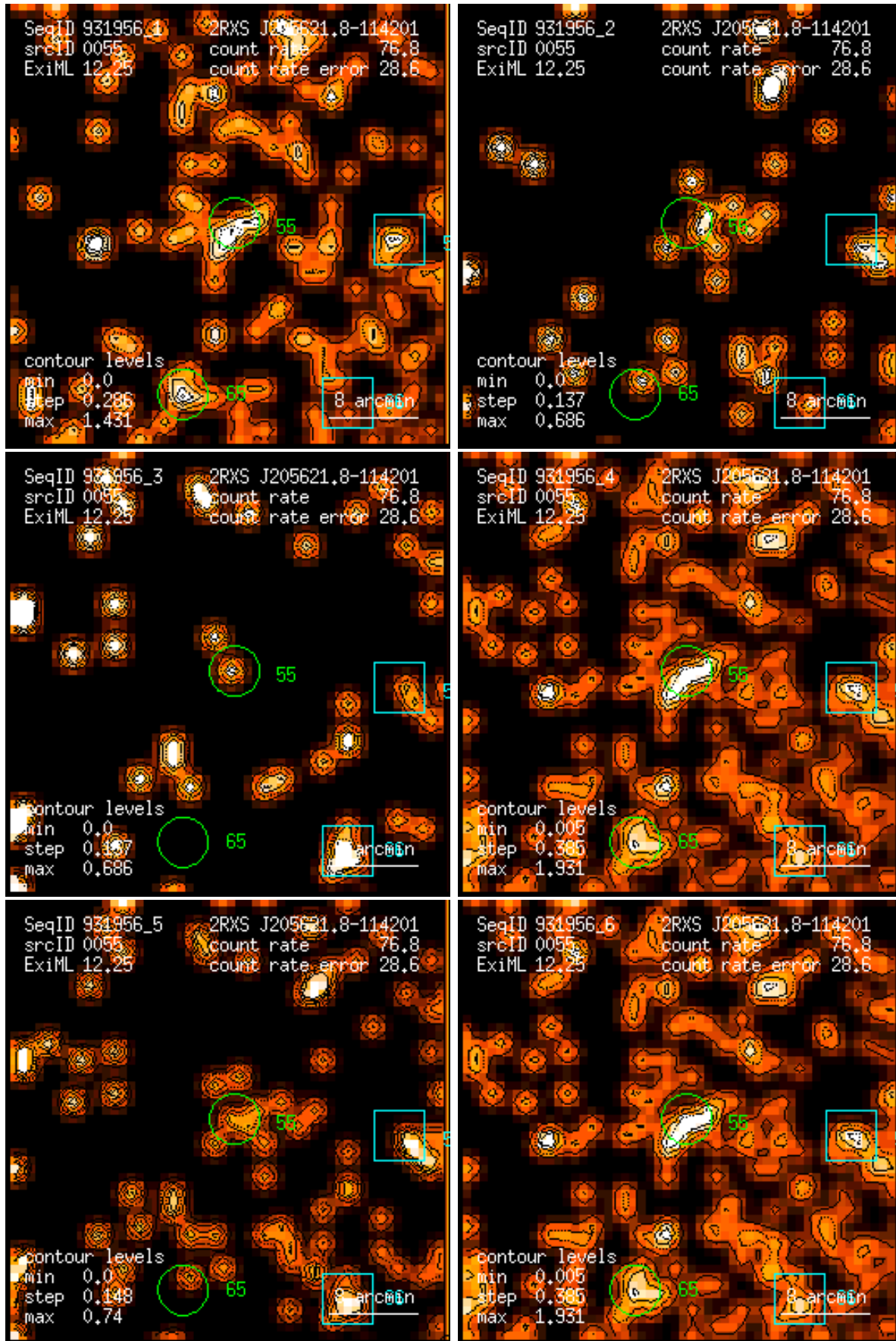
Figure 55: RASS 931956: detection 0055: band rate images, Gaussian filter: (1) PSPC channels 11 – 41, (2) 52 – 90, (3) 91 – 201, (4) 11 – 235, (5) 52 – 201, (6) 11 – 201. Broad band rates in counts/ks. Band rate contour levels in counts/ks/arcmin 2 .
