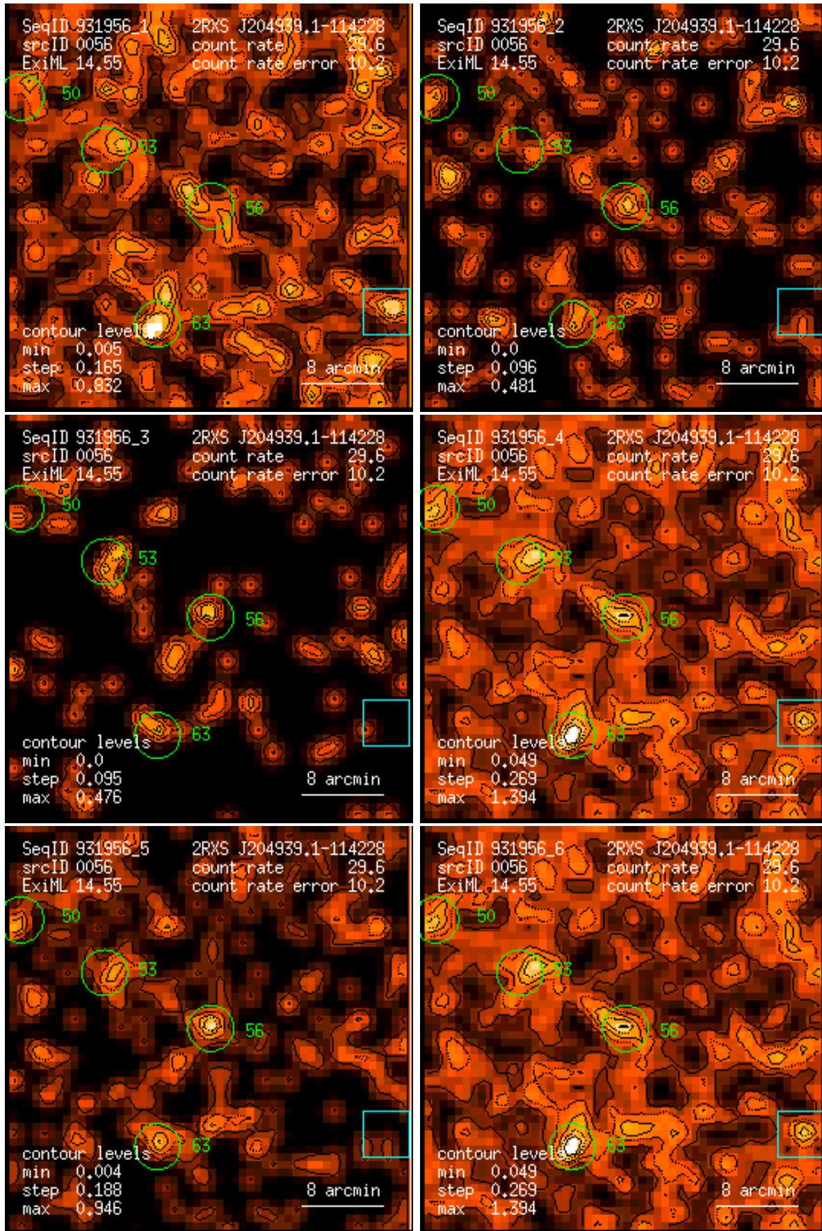
Figure 56: RASS 931956: detection 0056: band rate images, Gaussian filter: (1) PSPC channels 11 – 41, (2) 52 – 90, (3) 91 – 201, (4) 11 – 235, (5) 52 – 201, (6) 11 – 201. Broad band rates in counts/ks. Band rate contour levels in counts/ks/arcmin 2 .
