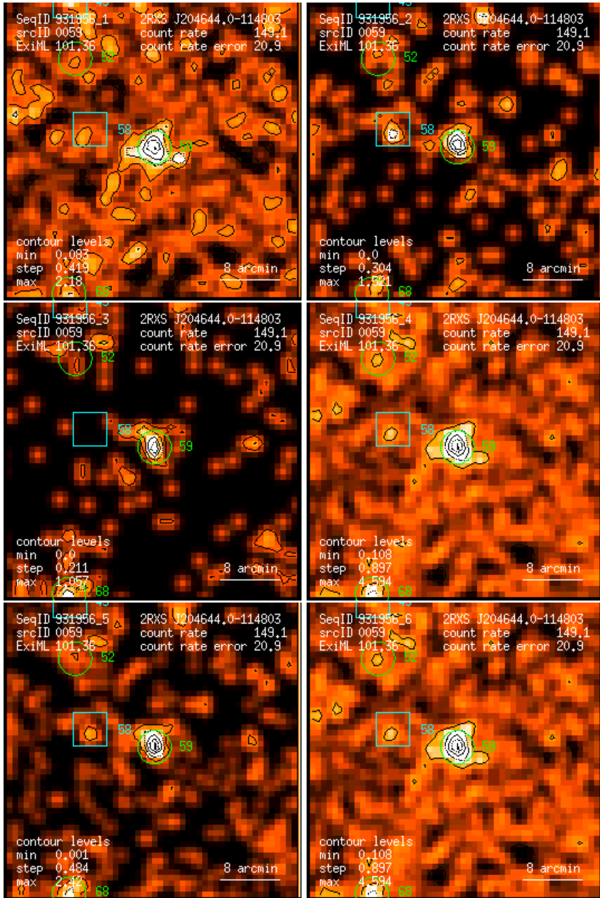
Figure 59: RASS 931956: detection 0059: band rate images, Gaussian filter: (1) PSPC channels 11 – 41, (2) 52 – 90, (3) 91 – 201, (4) 11 – 235, (5) 52 – 201, (6) 11 – 201. Broad band rates in counts/ks. Band rate contour levels in counts/ks/arcmin 2 .
