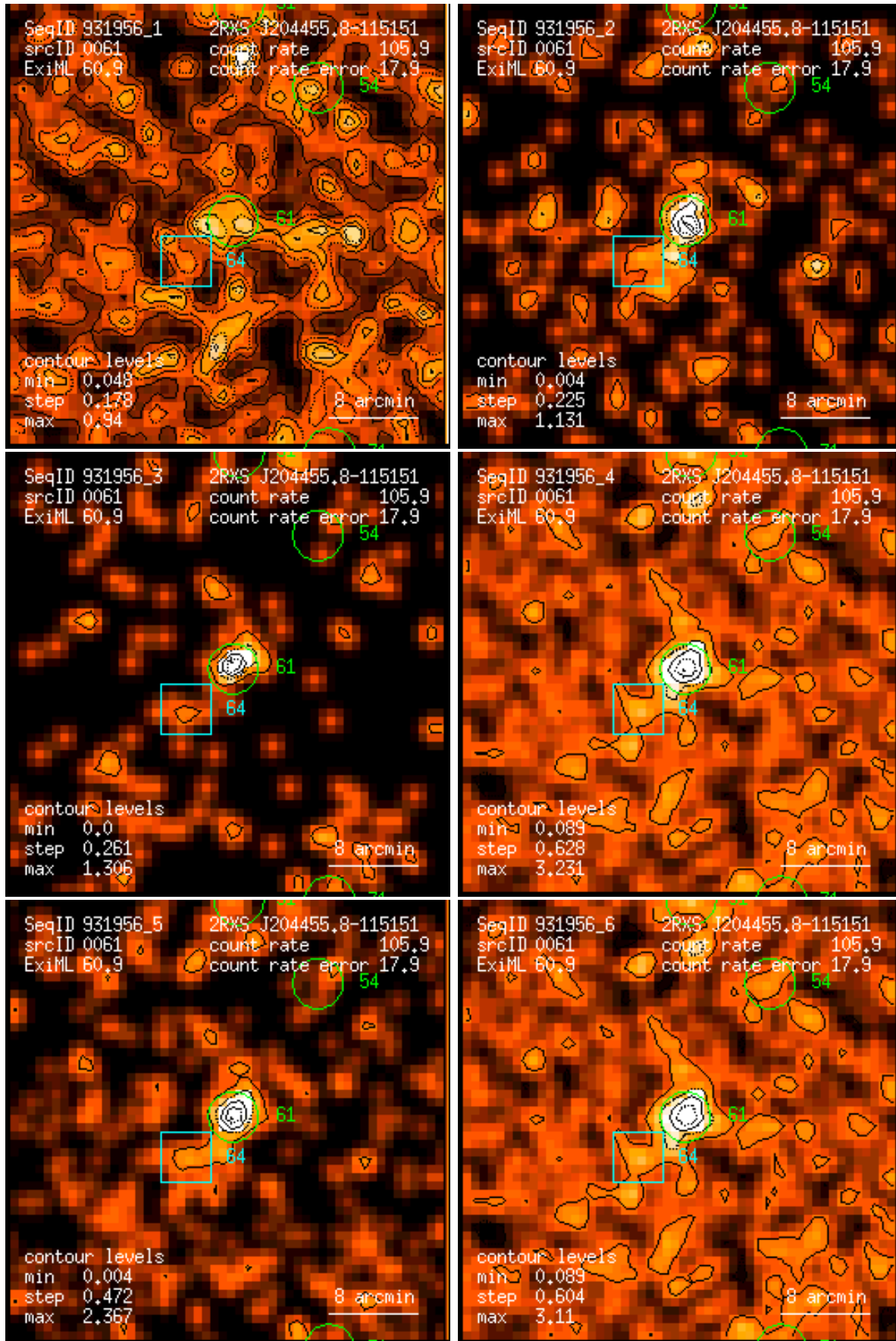
Figure 61: RASS 931956: detection 0061: band rate images, Gaussian filter: (1) PSPC channels 11 – 41, (2) 52 – 90, (3) 91 – 201, (4) 11 – 235, (5) 52 – 201, (6) 11 – 201. Broad band rates in counts/ks. Band rate contour levels in counts/ks/arcmin 2 .
